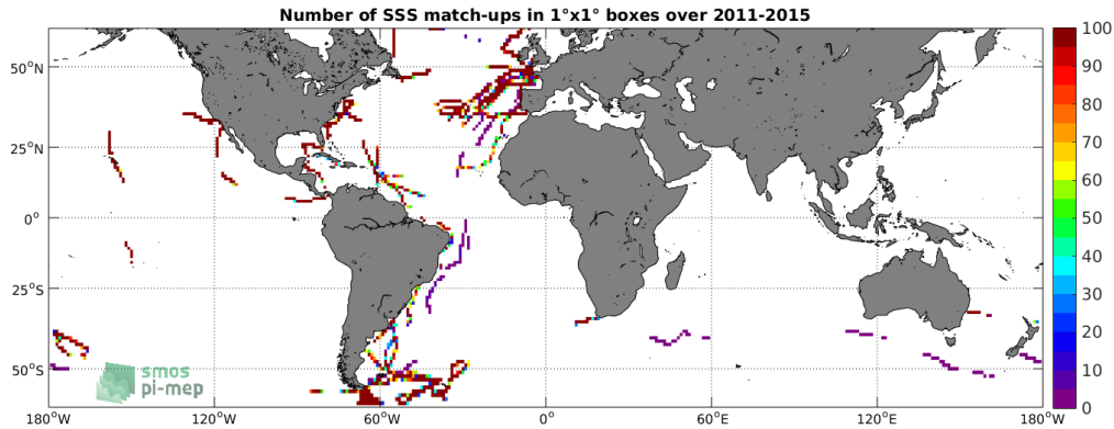
Figure 4: Number of SSS match-ups between TSG (GOSUD-Sailing-ship) SSS and the Aquarius SSS L4 OI v5 - Weekly (IPRC) SSS product for the SMOS coastal zone (<800km) 60N-60S Pi-MEP region over 1^\circ \times 1^\circ boxes and for the full satellite product period.
