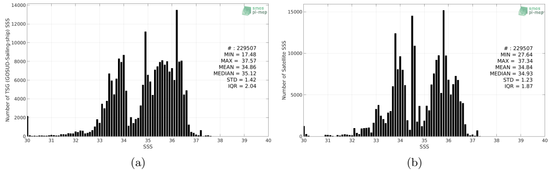
Figure 2: Histograms of SSS from TSG (GOSUD-Sailing-ship) (a) and Aquarius SSS L4 OI v5 - Weekly (IPRC) (b) considering all match-up pairs per bins of 0.1 over the SMOS coastal zone (<800km) 60N-60S Pi-MEP region and for the full satellite product period.
