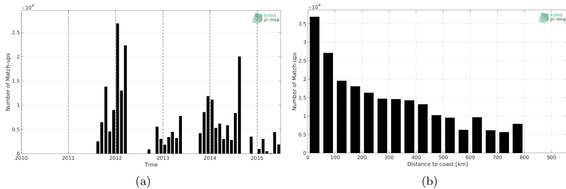
Figure 1: Number of match-ups between TSG (GOSUD-Sailing-ship) and Aquarius SSS L4 OI v5 - Weekly (IPRC) SSS as a function of time (a) and as function of the distance to coast (b) over the SMOS coastal zone (<800km) 60N-60S Pi-MEP region and for the full satellite product period.
