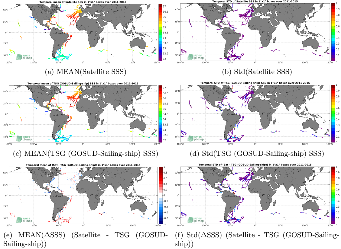
Figure 6: Temporal mean (left) and Std (right) of SSS from Aquarius SSS L4 OI v5 - Weekly (IPRC) (top), TSG (GOSUD-Sailing-ship) (middle), and of \Delta SSS (Satellite - TSG (GOSUD-Sailing-ship)). Only match-up pairs are used to generate these maps.
