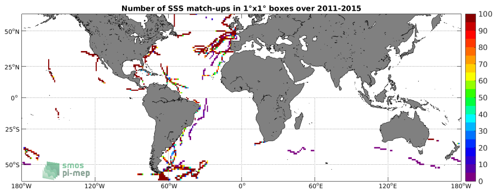
Figure 4: Number of SSS match-ups between TSG (GOSUD-Sailing-ship) SSS and the Aquarius SSS L4 OI v5 - Weekly (IPRC) SSS product for the SMOS coastal zone (<800km) 60N-60S Pi-MEP region over 1°x1° boxes and for the full satellite product period.
