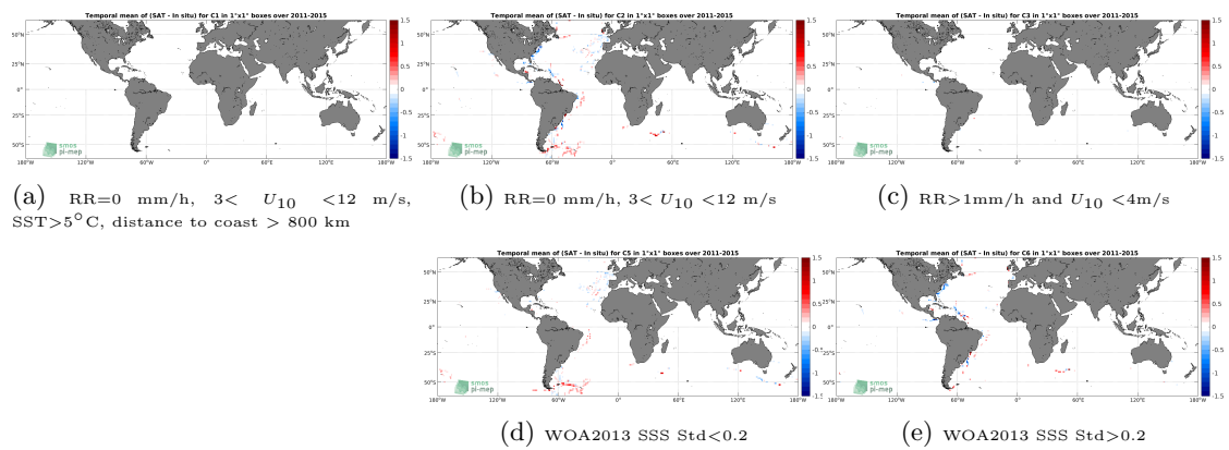
Figure 12: Temporal mean gridded over spatial boxes of size 1°x1° of \Delta SSS (Aquarius SSS L4 OI v5 - Weekly (IPRC) - TSG (GOSUD-Sailing-ship)) for 5 different subdatasets corresponding to:RR=0 mm/h, 3 < U_{10} < 12 m/s, SST>5°C, distance to coast > 800 km (a), RR=0 mm/h, 3 < U_{10} < 12 m/s (b), RR>1mm/h and U_{10} < 4 m/s (c), WOA2013 SSS Std<0.2 (d), WOA2013 SSS Std>0.2 (e).
