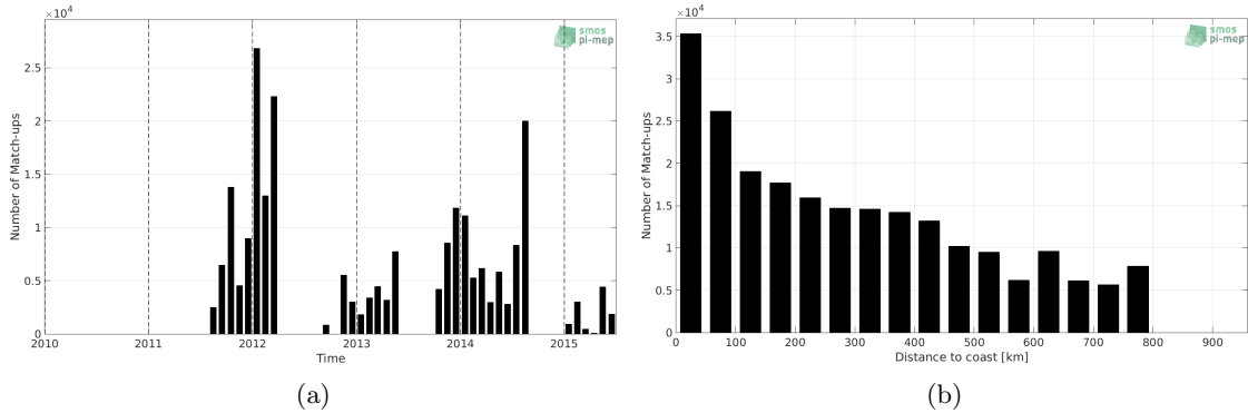
Figure 1: Number of match-ups between TSG-GOSUD-Sailing-ship and Aquarius-L4-IPRC-V5-WEEKLY SSS as a function of time (a) and as function of the distance to coast (b) over the SMOS coastal zone (<800km) 60N-60S Pi-MEP region and for the full satellite product period.
