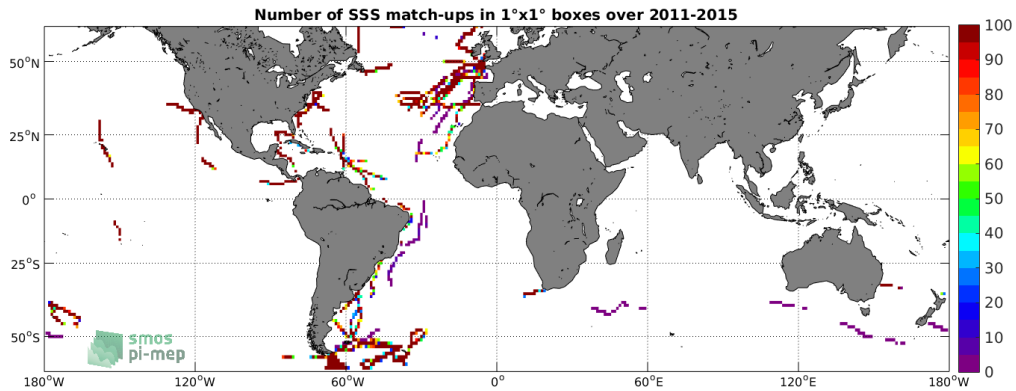
Figure 4: Number of SSS match-ups between TSG-GOSUD-Sailing-ship SSS and the Aquarius-L4-IPRC-V5-WEEKLY SSS product for the SMOS coastal zone (<800km) 60N-60S Pi-MEP region over 1^\circ \times 1^\circ boxes and for the full satellite product period.
