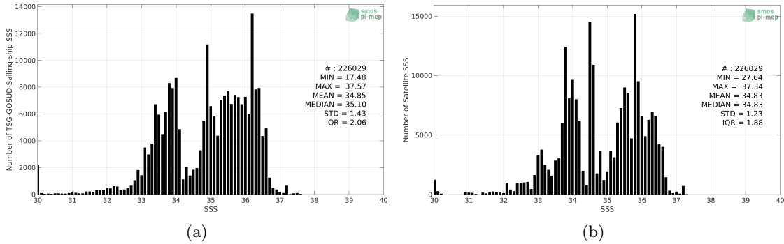
Figure 2: Histograms of SSS from TSG-GOSUD-Sailing-ship (a) and Aquarius-L4-IPRC-V5-WEEKLY (b) considering all match-up pairs per bins of 0.1 over the SMOS coastal zone (<800km) 60N-60S Pi-MEP region and for the full satellite product period.
