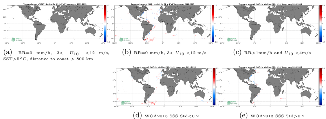
Figure 12: Temporal mean gridded over spatial boxes of size 1^\circ \times 1^\circ of \Delta SSS (Aquarius-L4-IPRC-V5-WEEKLY - TSG-GOSUD-Sailing-ship) for 5 different subdatasets corresponding to:RR=0 mm/h, 3 < U_{10} < 12 m/s, SST >5^\circ C, distance to coast > 800 km (a), RR=0 mm/h, 3 < U_{10} < 12 m/s (b), RR >1 mm/h and U_{10} < 4 m/s (c), WOA2013 SSS Std <0.2 (d), WOA2013 SSS Std >0.2 (e).
