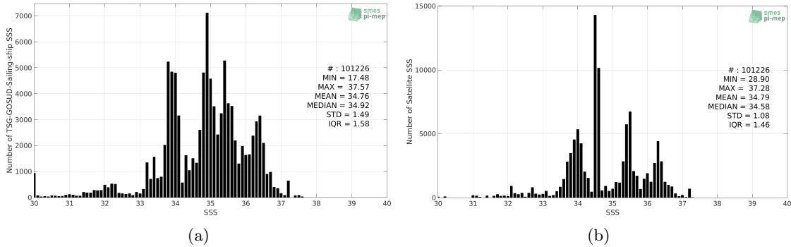
Figure 2: Histograms of SSS from TSG-GOSUD-Sailing-ship (a) and Aquarius-L4-IPRC-V5-WEEKLY (b) considering all match-up pairs per bins of 0.1 over the SMOS coastal zone ( \pm 800\text{km} ) 60N-60S Pi-MEP region and for the full satellite product period.
