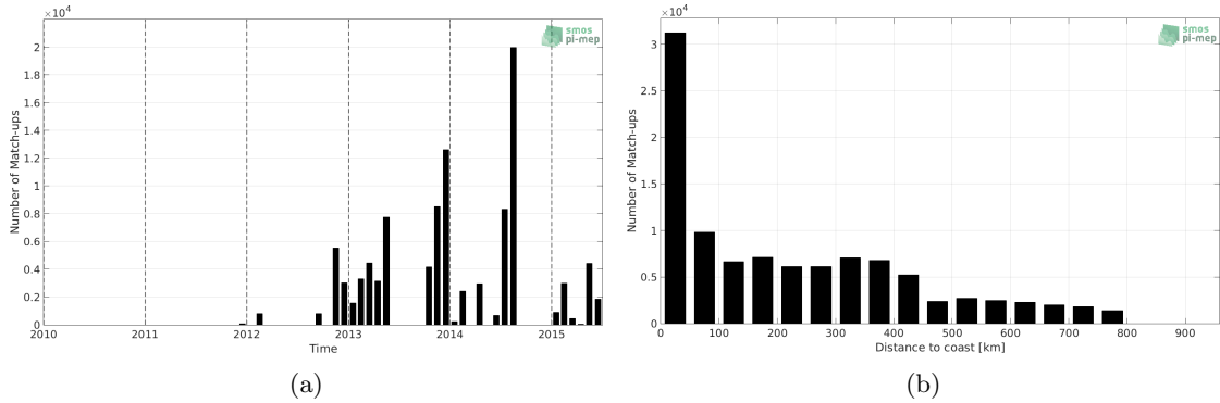
Figure 1: Number of match-ups between TSG-GOSUD-Sailing-ship and Aquarius-L4-IPRC-V5-WEEKLY SSS as a function of time (a) and as function of the distance to coast (b) over the SMOS coastal zone ( \pm 800\text{km} ) 60N-60S Pi-MEP region and for the full satellite product period.
