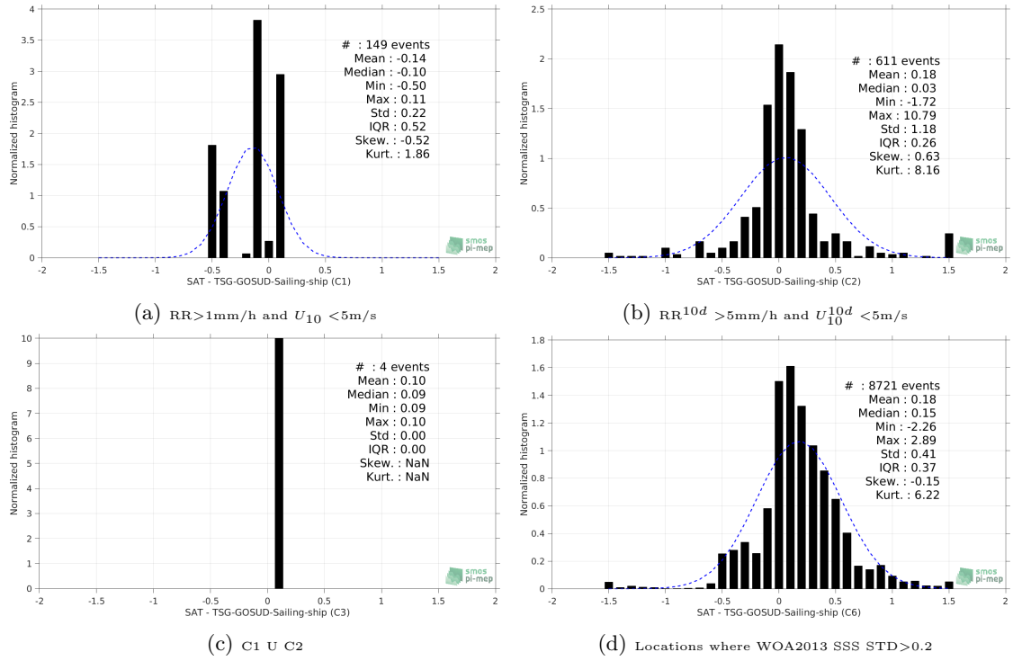
Figure 13: Normalized histogram of \Delta\text{SSS} (Aquarius-L4-IPRC-V5-WEEKLY - TSG-GOSUD-Sailing-ship) for 6 different subdatasets corresponding to: RR > 1mm/h and U_{10} < 5\text{m/s} (a), \text{RR}^{10d} > 5\text{mm/h} and U_{10}^{10d} < 5\text{m/s} (b), C1 U C2 (c), Locations where WOA2013 SSS STD > 0.2 (d).
