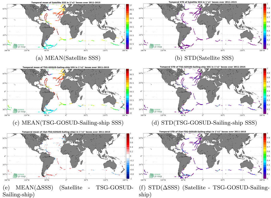
Figure 6: Temporal mean (left) and STD (right) of SSS from Aquarius-L4-IPRC-V5-WEEKLY (top), TSG-GOSUD-Sailing-ship (middle), and of \Delta SSS (Satellite - TSG-GOSUD-Sailing-ship). Only match-up pairs are used to generate these maps.
