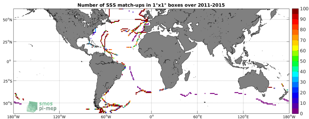
Figure 4: Number of SSS match-ups between TSG-GOSUD-Sailing-ship SSS and the Aquarius-L4-IPRC-V5-WEEKLY SSS product for the SMOS coastal zone ( \pm 800\text{km} ) 60N-60S Pi-MEP region over 1^\circ \times 1^\circ boxes and for the full satellite product period.
