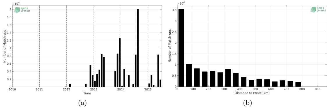
Figure 1: Number of match-ups between TSG-GOSUD-Sailing-ship and Aquarius-L4-IPRC-V5-WEEKLY SSS as a function of time (a) and as function of the distance to coast (b) over the SMOS coastal zone ( \approx 800\text{km} ) 60N-60S Pi-MEP region and for the full satellite product period.
