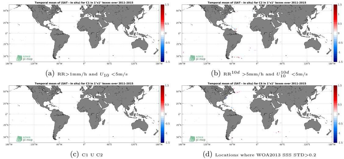
Figure 12: Temporal mean gridded over spatial boxes of size 1^\circ \times 1^\circ of \Delta SSS (Aquarius-L4-IPRC-V5-WEEKLY - TSG-GOSUD-Sailing-ship) for 4 different subdatasets corresponding to: RR > 1\text{mm/h} and U_{10} < 5\text{m/s} (a), RR^{10d} > 5\text{mm/h} and U_{10}^{10d} < 5\text{m/s} (b), C1 U C2 (c), Locations where WOA2013 SSS STD > 0.2 (d).
