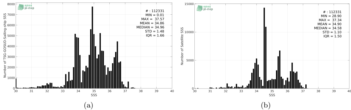
Figure 2: Histograms of SSS from TSG-GOSUD-Sailing-ship (a) and Aquarius-L4-IPRC-V5-WEEKLY (b) considering all match-up pairs per bins of 0.1 over the SMOS coastal zone ( \approx 800\text{km} ) 60N-60S Pi-MEP region and for the full satellite product period.
