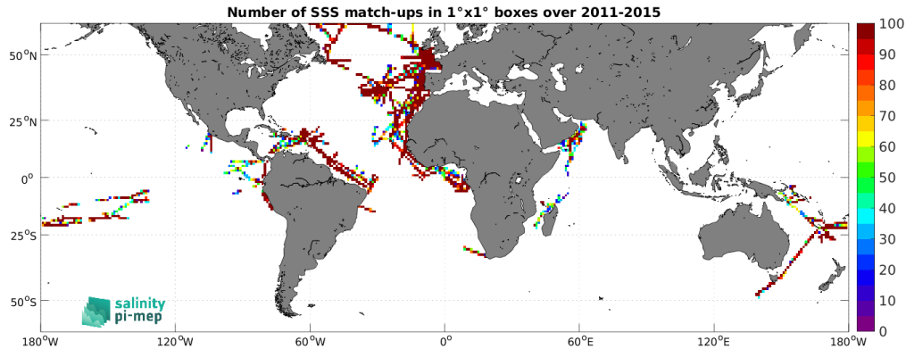
Figure 5: Number of SSS match-ups between TSG (GOSUD-Research-vessel) SSS and the Aquarius SSS L4 OI v5 - Weekly (IPRC) SSS product for the SMOS coastal zone (<800km) 60N-60S Pi-MEP region over 1^{\circ} \times 1^{\circ} boxes and for the full satellite product period.
