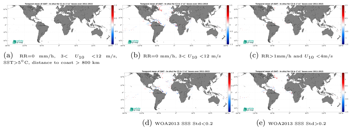
Figure 14: Temporal mean gridded over spatial boxes of size 1^\circ \times 1^\circ of \Delta\text{SSS} (Aquarius SSS L4 OI v5 - Weekly (IPRC) - TSG (GOSUD-Research-vessel)) for 5 different subdatasets corresponding to:RR=0 mm/h, 3 < U_{10} < 12 m/s, SST >5^\circ\text{C} , distance to coast > 800 km (a), RR=0 mm/h, 3 < U_{10} < 12 m/s (b), RR >1 mm/h and U_{10} < 4 m/s (c), WOA2013 SSS Std <0.2 (d), WOA2013 SSS Std >0.2 (e).
