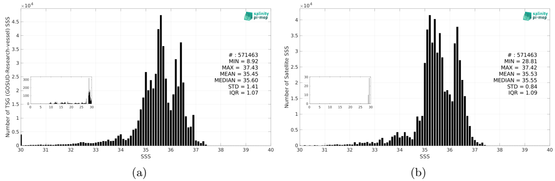
Figure 3: Histograms of SSS from TSG (GOSUD-Research-vessel) (a) and Aquarius SSS L4 OI v5 - Weekly (IPRC) (b) considering all match-up pairs per bins of 0.1 over the SMOS coastal zone (<800km) 60N-60S Pi-MEP region and for the full satellite product period.
