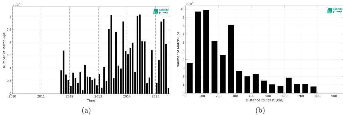
Figure 2: Number of match-ups between TSG (GOSUD-Research-vessel) and Aquarius SSS L4 OI v5 - Weekly (IPRC) SSS as a function of time (a) and as function of the distance to coast (b) over the SMOS coastal zone (<800km) 60N-60S Pi-MEP region and for the full satellite product period.
