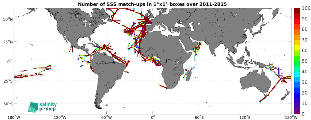
Figure 4: Number of SSS match-ups between TSG (GOSUD-Research-vessel) SSS and the Aquarius SSS L4 OI v5 - Weekly (IPRC) SSS product for the SMOS coastal zone (<800km) 60N-60S Pi-MEP region over 1^\circ \times 1^\circ boxes and for the full satellite product period.
