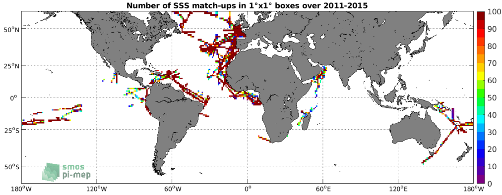
Figure 4: Number of SSS match-ups between TSG (GOSUD-Research-vessel) SSS and the Aquarius SSS L4 OI v5 - Weekly (IPRC) SSS product for the SMOS coastal zone (<800km) 60N-60S Pi-MEP region over 1^{\circ} \times 1^{\circ} boxes and for the full satellite product period.
