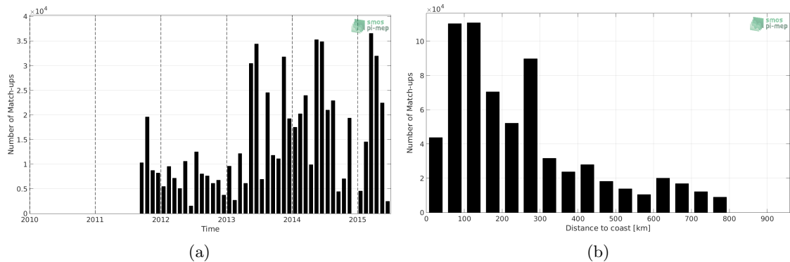
Figure 1: Number of match-ups between TSG-GOSUD-Research-vessel and Aquarius-L4-IPRC-V5-WEEKLY SSS as a function of time (a) and as function of the distance to coast (b) over the SMOS coastal zone (<800km) 60N-60S Pi-MEP region and for the full satellite product period.
