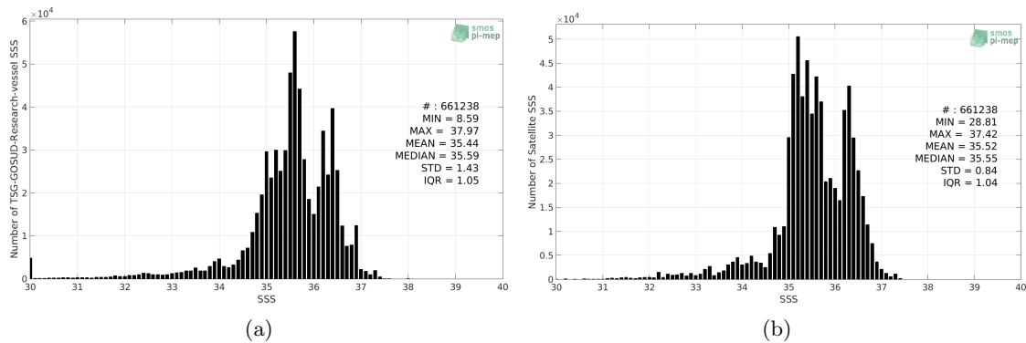
Figure 2: Histograms of SSS from TSG-GOSUD-Research-vessel (a) and Aquarius-L4-IPRC-V5-WEEKLY (b) considering all match-up pairs per bins of 0.1 over the SMOS coastal zone (<800km) 60N-60S Pi-MEP region and for the full satellite product period.
