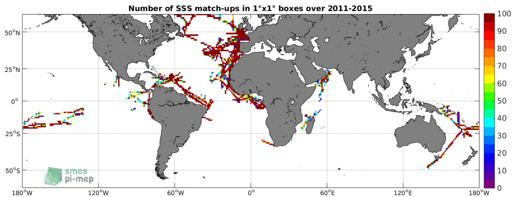
Figure 4: Number of SSS match-ups between TSG-GOSUD-Research-vessel SSS and the Aquarius-L4-IPRC-V5-WEEKLY SSS product for the SMOS coastal zone (<800km) 60N-60S Pi-MEP region over 1°x1° boxes and for the full satellite product period.
