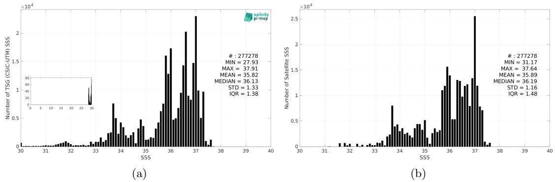
Figure 3: Histograms of SSS from TSG (CSIC-UTM) (a) and Aquarius SSS L4 OI v5 - Weekly (IPRC) (b) considering all match-up pairs per bins of 0.1 over the SMOS coastal zone (<800km) 60N-60S Pi-MEP region and for the full satellite product period.
