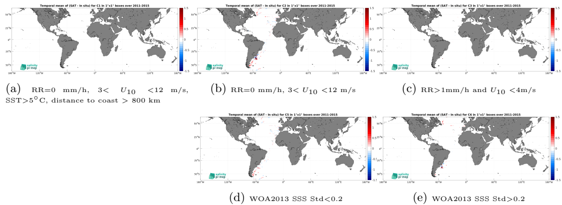
Figure 12: Temporal mean gridded over spatial boxes of size 1^\circ \times 1^\circ of \Delta\text{SSS} (Aquarius SSS L4 OI v5 - Weekly (IPRC) - TSG (CSIC-UTM)) for 5 different subdatasets corresponding to:RR=0 mm/h, 3 < U_{10} < 12 m/s, SST >5^\circ\text{C} , distance to coast > 800 km (a), RR=0 mm/h, 3 < U_{10} < 12 m/s (b), RR >1 mm/h and U_{10} < 4 m/s (c), WOA2013 SSS Std <0.2 (d), WOA2013 SSS Std >0.2 (e).
