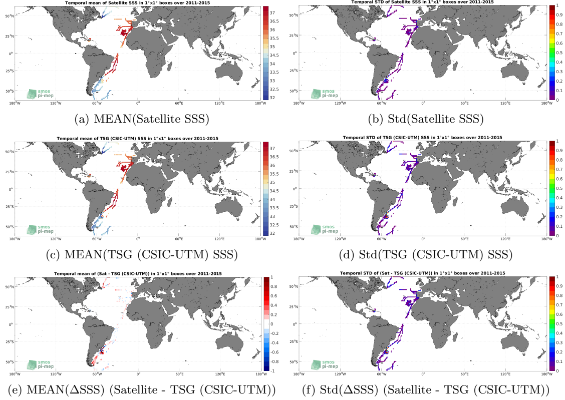
Figure 6: Temporal mean (left) and Std (right) of SSS from Aquarius SSS L4 OI v5 - Weekly (IPRC) (top), TSG (CSIC-UTM) (middle), and of \Delta SSS (Satellite - TSG (CSIC-UTM)). Only match-up pairs are used to generate these maps.
