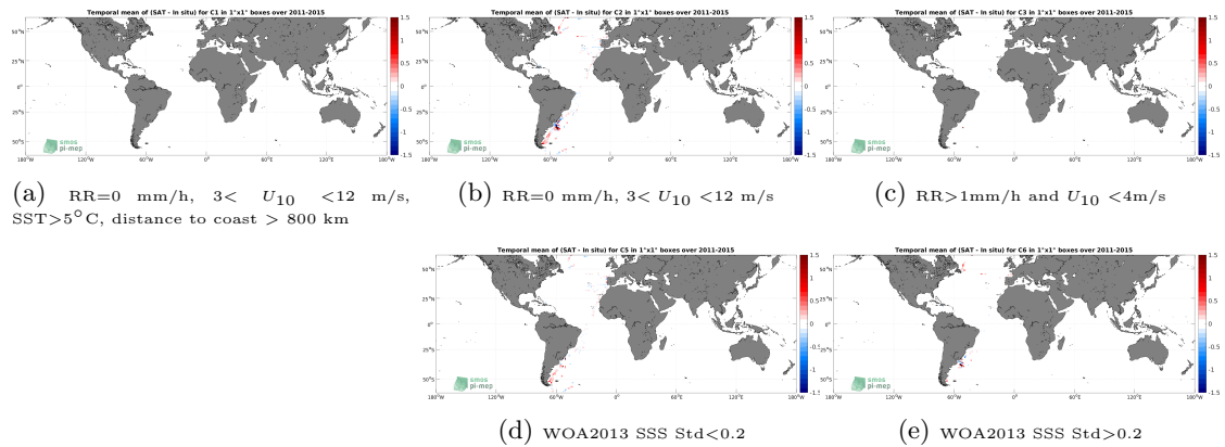
Figure 12: Temporal mean gridded over spatial boxes of size 1^\circ \times 1^\circ of \Delta SSS (Aquarius SSS L4 OI v5 - Weekly (IPRC) - TSG (CSIC-UTM)) for 5 different subdatasets corresponding to:RR=0 mm/h, 3 < U_{10} < 12 m/s, SST >5^\circ\text{C} , distance to coast > 800 km (a), RR=0 mm/h, 3 < U_{10} < 12 m/s (b), RR >1 mm/h and U_{10} < 4 m/s (c), WOA2013 SSS Std <0.2 (d), WOA2013 SSS Std >0.2 (e).
