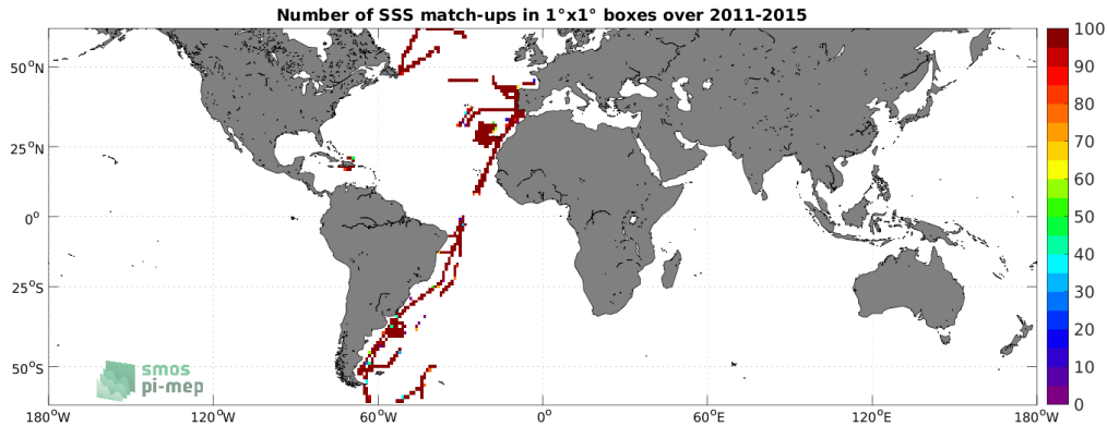
Figure 4: Number of SSS match-ups between TSG (CSIC-UTM) SSS and the Aquarius SSS L4 OI v5 - Weekly (IPRC) SSS product for the SMOS coastal zone (<800km) 60N-60S Pi-MEP region over 1^{\circ} \times 1^{\circ} boxes and for the full satellite product period.
