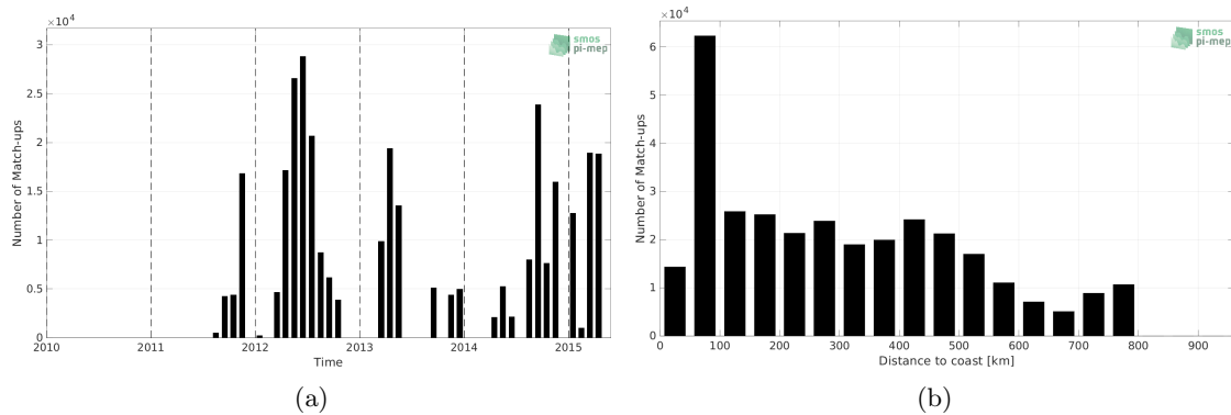
Figure 1: Number of match-ups between TSG (CSIC-UTM) and Aquarius SSS L4 OI v5 - Weekly (IPRC) SSS as a function of time (a) and as function of the distance to coast (b) over the SMOS coastal zone (<800km) 60N-60S Pi-MEP region and for the full satellite product period.
