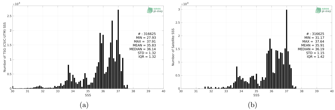
Figure 2: Histograms of SSS from TSG (CSIC-UTM) (a) and Aquarius SSS L4 OI v5 - Weekly (IPRC) (b) considering all match-up pairs per bins of 0.1 over the SMOS coastal zone (<800km) 60N-60S Pi-MEP region and for the full satellite product period.
