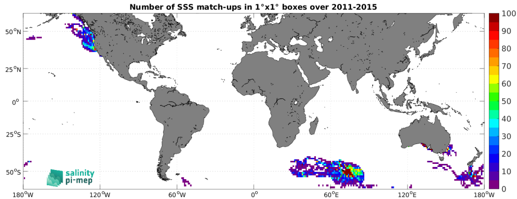
Figure 5: Number of SSS match-ups between Marine mammals SSS and the Aquarius SSS L4 OI v5 - Weekly (IPRC) SSS product for the SMOS coastal zone (<800km) 60N-60S Pi-MEP region over 1^\circ \times 1^\circ boxes and for the full satellite product period.
