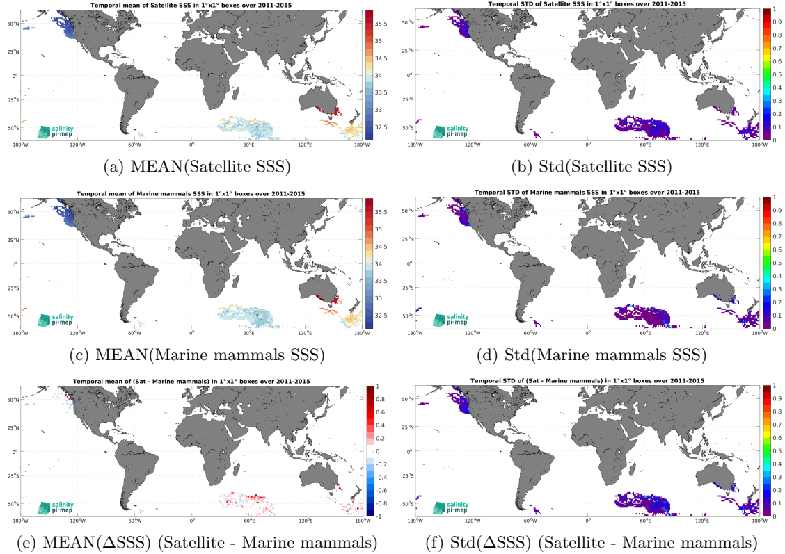
Figure 7: Temporal mean (left) and Std (right) of SSS from Aquarius SSS L4 OI v5 - Weekly (IPRC) (top), Marine mammals (middle), and of \Delta SSS (Satellite - Marine mammals). Only match-up pairs are used to generate these maps.
