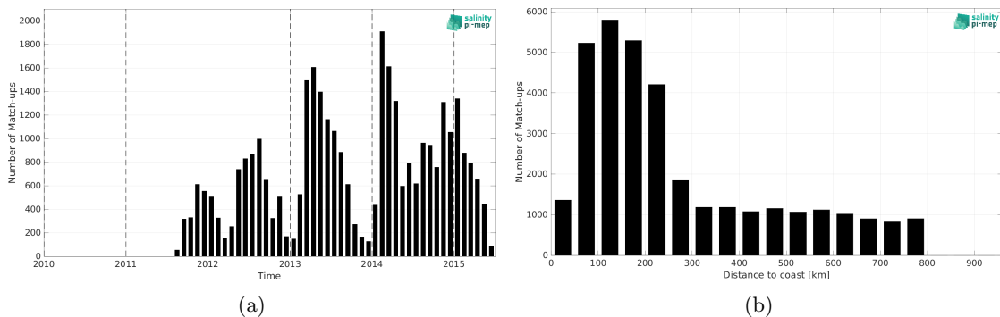
Figure 2: Number of match-ups between Marine mammals and Aquarius SSS L4 OI v5 - Weekly (IPRC) SSS as a function of time (a) and as function of the distance to coast (b) over the SMOS coastal zone (<800km) 60N-60S Pi-MEP region and for the full satellite product period.
