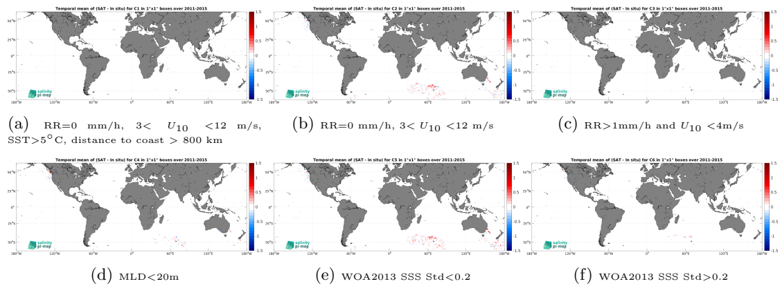
Figure 14: Temporal mean gridded over spatial boxes of size 1^\circ \times 1^\circ of \Delta SSS (Aquarius SSS L4 OI v5 - Weekly (IPRC) - Marine mammals) for 6 different subdatasets corresponding to:RR=0 mm/h, 3 < U_{10} < 12 m/s, SST >5^\circ C, distance to coast > 800 km (a), RR=0 mm/h, 3 < U_{10} < 12 m/s (b), RR >1 mm/h and U_{10} < 4 m/s (c),MLD <20 m (d),WOA2013 SSS Std <0.2 (e),WOA2013 SSS Std >0.2 (f).
