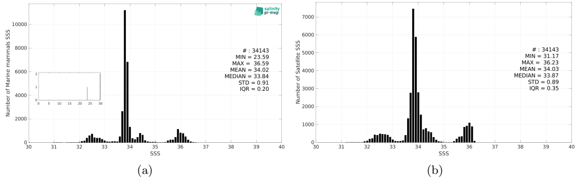
Figure 3: Histograms of SSS from Marine mammals (a) and Aquarius SSS L4 OI v5 - Weekly (IPRC) (b) considering all match-up pairs per bins of 0.1 over the SMOS coastal zone (<800km) 60N-60S Pi-MEP region and for the full satellite product period.
