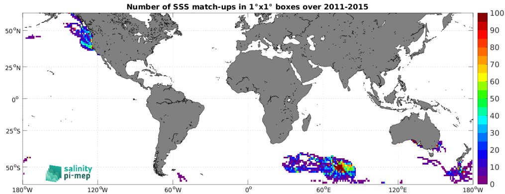
Figure 4: Number of SSS match-ups between Marine mammals SSS and the Aquarius SSS L4 OI v5 - Weekly (IPRC) SSS product for the SMOS coastal zone (<800km) 60N-60S Pi-MEP region over 1^{\circ} \times 1^{\circ} boxes and for the full satellite product period.
