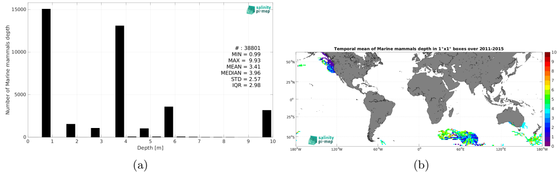
Figure 3: Histograms of the depth of the upper level SSS measurements from Marine mammals in the Match-up DataBase for the SMOS coastal zone (<800km) 60N-60S Pi-MEP region (a) and temporal mean spatial distribution of pressure of the in situ SSS data over 1^\circ \times 1^\circ boxes and for the full satellite product period (b).
