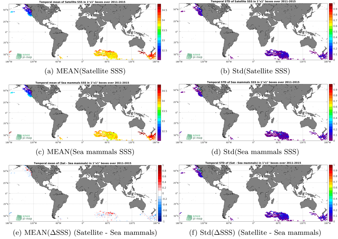
Figure 6: Temporal mean (left) and Std (right) of SSS from Aquarius-L4-IPRC-V5-WEEKLY (top), Sea mammals (middle), and of \Delta SSS (Satellite - Sea mammals). Only match-up pairs are used to generate these maps.
