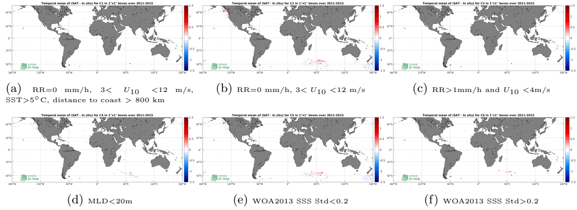
Figure 12: Temporal mean gridded over spatial boxes of size 1^\circ \times 1^\circ of \Delta SSS (Aquarius-L4-IPRC-V5-WEEKLY - Sea mammals) for 6 different subdatasets corresponding to: RR=0 mm/h, 3 < U_{10} < 12 m/s, SST > 5^\circ C , distance to coast > 800 km (a), RR=0 mm/h, 3 < U_{10} < 12 m/s (b), RR > 1 mm/h and U_{10} < 4 m/s (c), MLD < 20 m (d), WOA2013 SSS Std < 0.2 (e), WOA2013 SSS Std > 0.2 (f).
