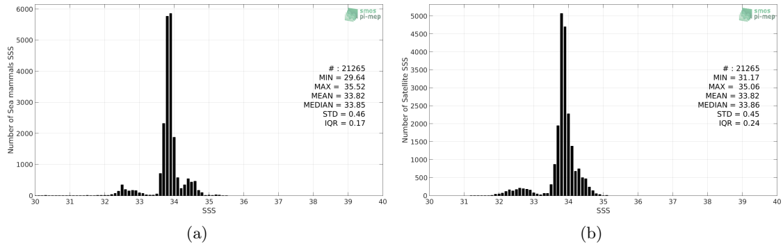
Figure 2: Histograms of SSS from Sea mammals (a) and Aquarius-L4-IPRC-V5-WEEKLY (b) considering all match-up pairs per bins of 0.1 over the SMOS coastal zone (<800km) 60N-60S Pi-MEP region and for the full satellite product period.
