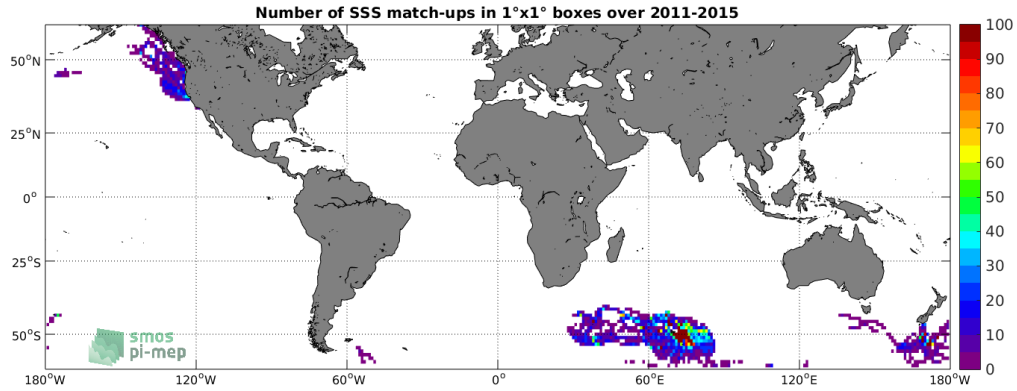
Figure 4: Number of SSS match-ups between Sea mammals SSS and the Aquarius-L4-IPRC-V5-WEEKLY SSS product for the SMOS coastal zone (<800km) 60N-60S Pi-MEP region over 1°x1° boxes and for the full satellite product period.
