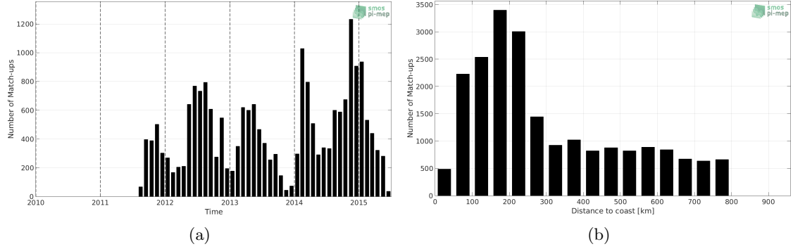
Figure 1: Number of match-ups between Sea mammals and Aquarius-L4-IPRC-V5-WEEKLY SSS as a function of time (a) and as function of the distance to coast (b) over the SMOS coastal zone (<800km) 60N-60S Pi-MEP region and for the full satellite product period.
