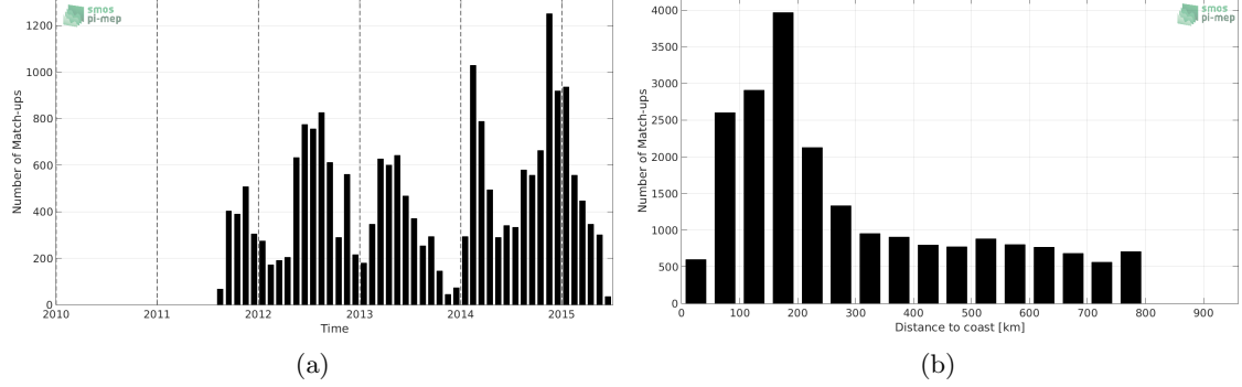
Figure 1: Number of match-ups between Sea mammals and Aquarius-L4-IPRC-V5-WEEKLY SSS as a function of time (a) and as function of the distance to coast (b) over the SMOS coastal zone ( \geq 800\text{km} ) 60N-60S Pi-MEP region and for the full satellite product period.
