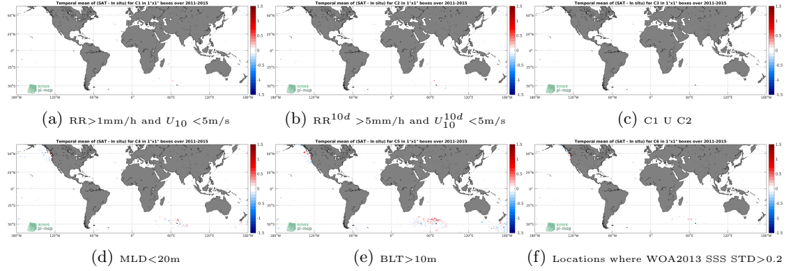
Figure 12: Temporal mean gridded over spatial boxes of size 1^\circ \times 1^\circ of \Delta SSS (Aquarius-L4-IPRC-V5-WEEKLY - Sea mammals) for 6 different subdatasets corresponding to: RR > 1\text{mm/h} and U_{10} < 5\text{m/s} (a), RR^{10d} > 5\text{mm/h} and U_{10}^{10d} < 5\text{m/s} (b), C1 U C2 (c), MLD < 20\text{m} (d), BLT > 10\text{m} (e), Locations where WOA2013 SSS STD > 0.2 (f).
