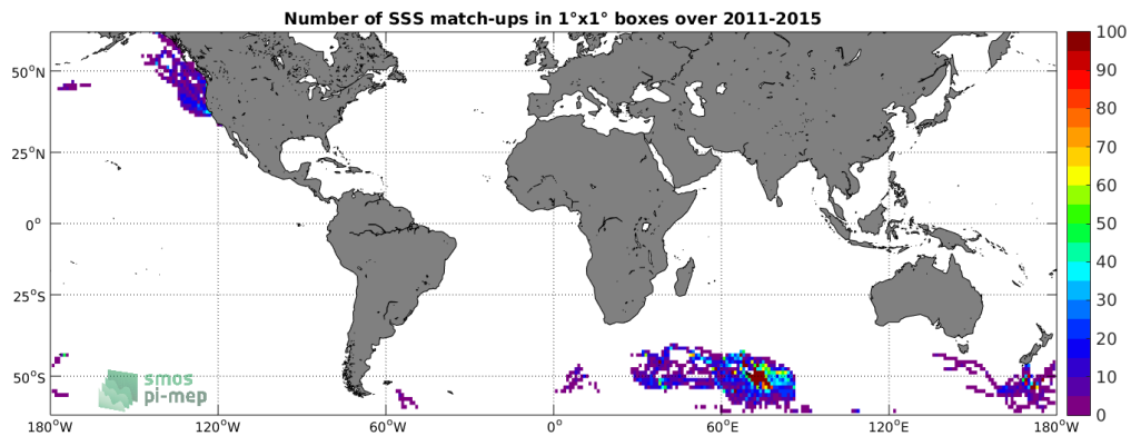
Figure 4: Number of SSS match-ups between Sea mammals SSS and the Aquarius-L4-IPRC-V5-WEEKLY SSS product for the SMOS coastal zone ( \pm 800\text{km} ) 60N-60S Pi-MEP region over 1^\circ \times 1^\circ boxes and for the full satellite product period.
