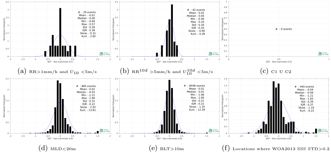
Figure 13: Normalized histogram of \Delta SSS (Aquarius-L4-IPRC-V5-WEEKLY - Sea mammals) for 6 different subdatasets corresponding to: RR > 1\text{mm/h} and U_{10} < 5\text{m/s} (a), RR^{10d} > 5\text{mm/h} and U_{10}^{10d} < 5\text{m/s} (b), C1 U C2 (c), MLD < 20\text{m} (d), BLT > 10\text{m} (e), Locations where WOA2013 SSS STD > 0.2 (f).
