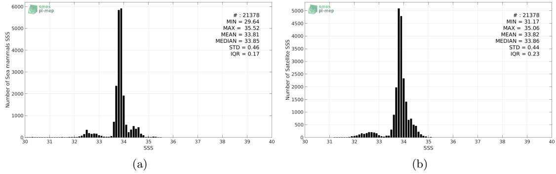
Figure 2: Histograms of SSS from Sea mammals (a) and Aquarius-L4-IPRC-V5-WEEKLY (b) considering all match-up pairs per bins of 0.1 over the SMOS coastal zone ( \geq 800\text{km} ) 60N-60S Pi-MEP region and for the full satellite product period.
