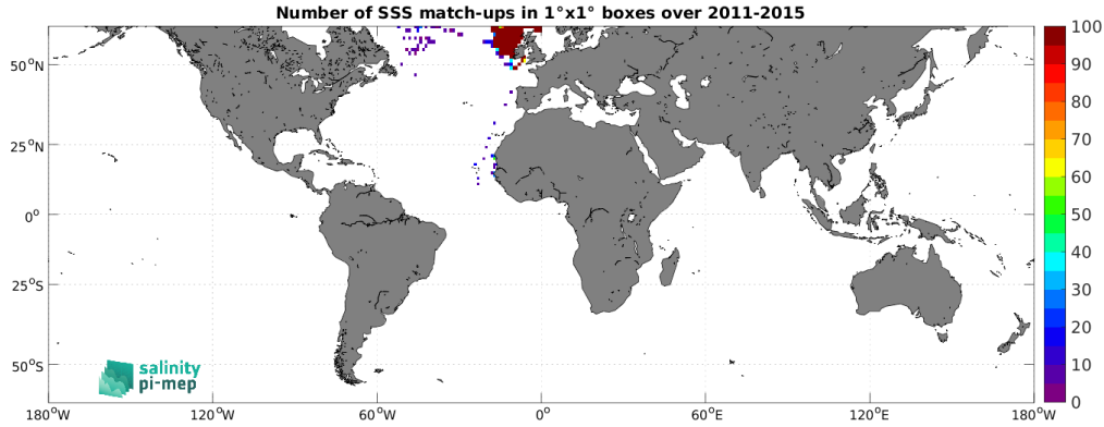
Figure 5: Number of SSS match-ups between ICES SSS and the Aquarius SSS L4 OI v5 - Weekly (IPRC) SSS product for the SMOS coastal zone (<800km) 60N-60S Pi-MEP region over 1^\circ \times 1^\circ boxes and for the full satellite product period.
