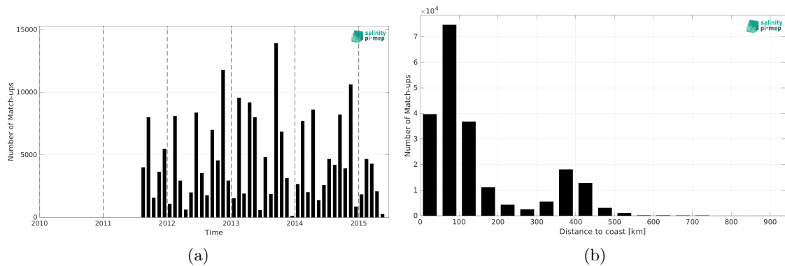
Figure 2: Number of match-ups between ICES and Aquarius SSS L4 OI v5 - Weekly (IPRC) SSS as a function of time (a) and as function of the distance to coast (b) over the SMOS coastal zone (<800km) 60N-60S Pi-MEP region and for the full satellite product period.
