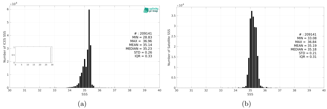
Figure 3: Histograms of SSS from ICES (a) and Aquarius SSS L4 OI v5 - Weekly (IPRC) (b) considering all match-up pairs per bins of 0.1 over the SMOS coastal zone (<800km) 60N-60S Pi-MEP region and for the full satellite product period.
