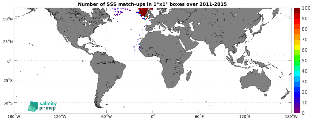
Figure 5: Number of SSS match-ups between ICES SSS and the Aquarius SSS L4 OI v5 - Weekly (IPRC) SSS product for the SMOS coastal zone ( <800\text{km} ) 60N-60S Pi-MEP region over 1^\circ \times 1^\circ boxes and for the full satellite product period.
