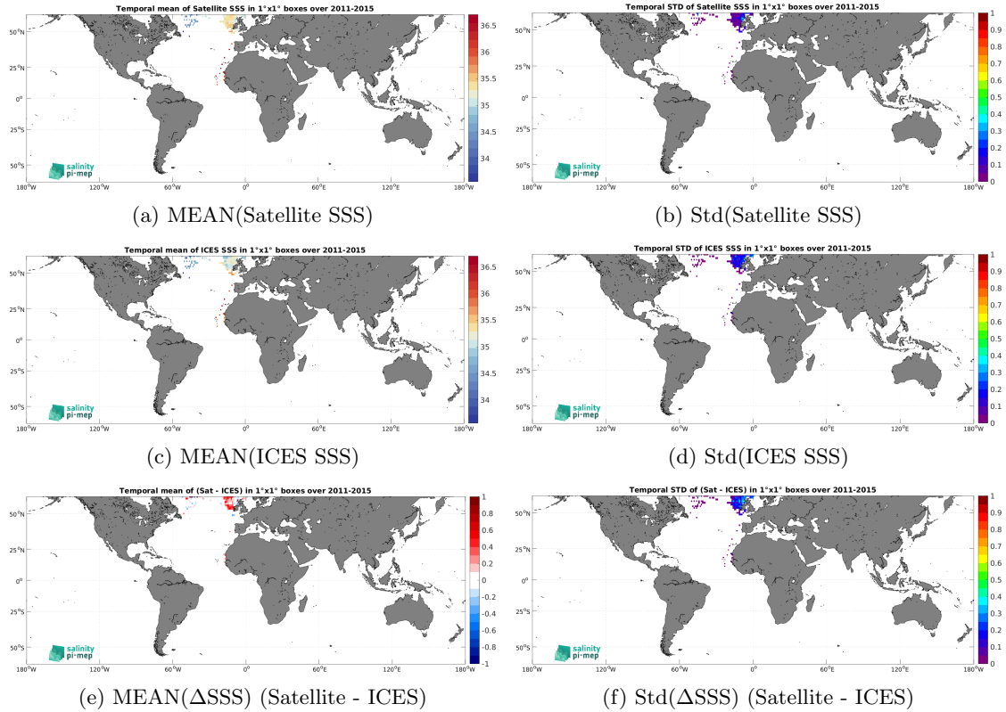
Figure 7: Temporal mean (left) and Std (right) of SSS from Aquarius SSS L4 OI v5 - Weekly (IPRC) (top), ICES (middle), and of \Delta SSS (Satellite - ICES). Only match-up pairs are used to generate these maps.
