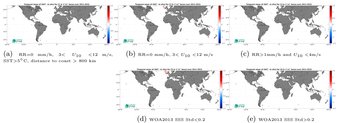
Figure 14: Temporal mean gridded over spatial boxes of size 1^\circ \times 1^\circ of \Delta SSS (Aquarius SSS L4 OI v5 - Weekly (IPRC) - ICES) for 5 different subdatasets corresponding to:RR=0 mm/h, 3 < U_{10} < 12 m/s, SST >5^\circ\text{C} , distance to coast > 800 km (a), RR=0 mm/h, 3 < U_{10} < 12 m/s (b), RR >1 mm/h and U_{10} < 4 m/s (c), WOA2013 SSS Std <0.2 (d), WOA2013 SSS Std >0.2 (e).
