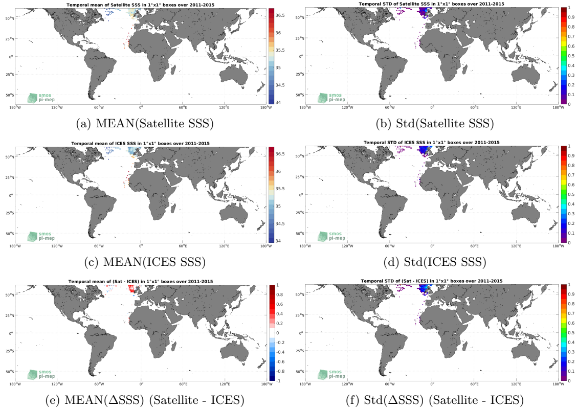
Figure 6: Temporal mean (left) and Std (right) of SSS from Aquarius SSS L4 OI v5 - Weekly (IPRC) (top), ICES (middle), and of \Delta SSS (Satellite - ICES). Only match-up pairs are used to generate these maps.
