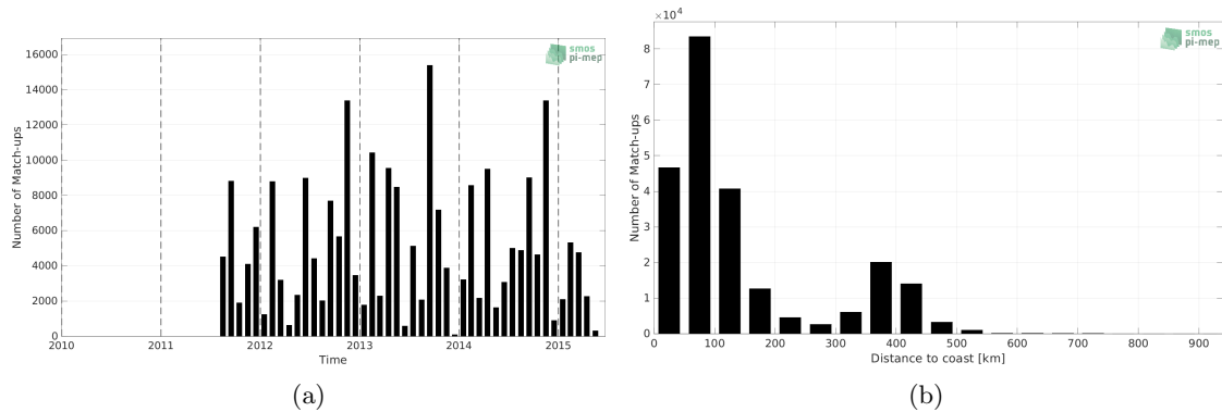
Figure 1: Number of match-ups between ICES and Aquarius SSS L4 OI v5 - Weekly (IPRC) SSS as a function of time (a) and as function of the distance to coast (b) over the SMOS coastal zone (<800km) 60N-60S Pi-MEP region and for the full satellite product period.
