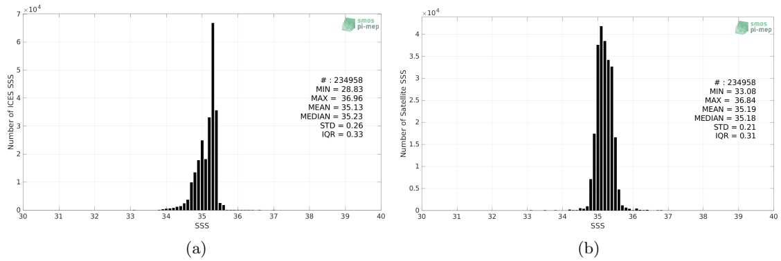
Figure 2: Histograms of SSS from ICES (a) and Aquarius SSS L4 OI v5 - Weekly (IPRC) (b) considering all match-up pairs per bins of 0.1 over the SMOS coastal zone (<800km) 60N-60S Pi-MEP region and for the full satellite product period.
