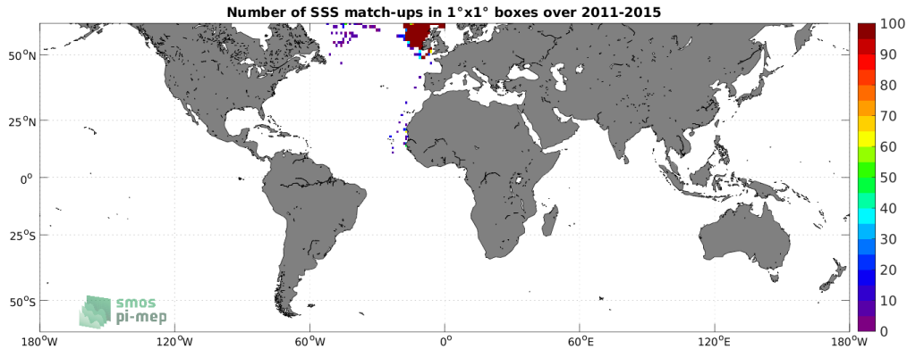
Figure 4: Number of SSS match-ups between ICES SSS and the Aquarius SSS L4 OI v5 - Weekly (IPRC) SSS product for the SMOS coastal zone (<800km) 60N-60S Pi-MEP region over 1^\circ \times 1^\circ boxes and for the full satellite product period.
