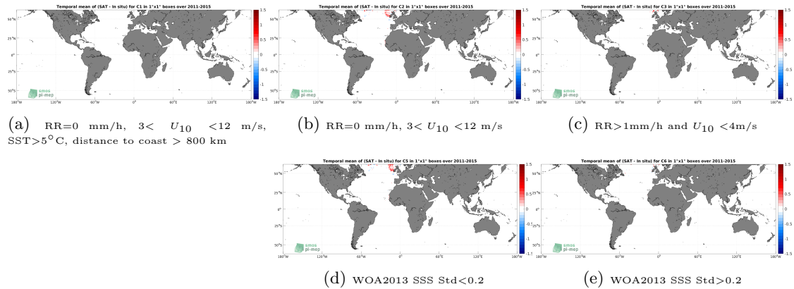
Figure 12: Temporal mean gridded over spatial boxes of size 1^\circ \times 1^\circ of \Delta SSS (Aquarius SSS L4 OI v5 - Weekly (IPRC) - ICES) for 5 different subdatasets corresponding to:RR=0 mm/h, 3 < U_{10} < 12 m/s, SST >5^\circ\text{C} , distance to coast > 800 km (a), RR=0 mm/h, 3 < U_{10} < 12 m/s (b), RR >1 mm/h and U_{10} < 4 m/s (c), WOA2013 SSS Std <0.2 (d), WOA2013 SSS Std >0.2 (e).
