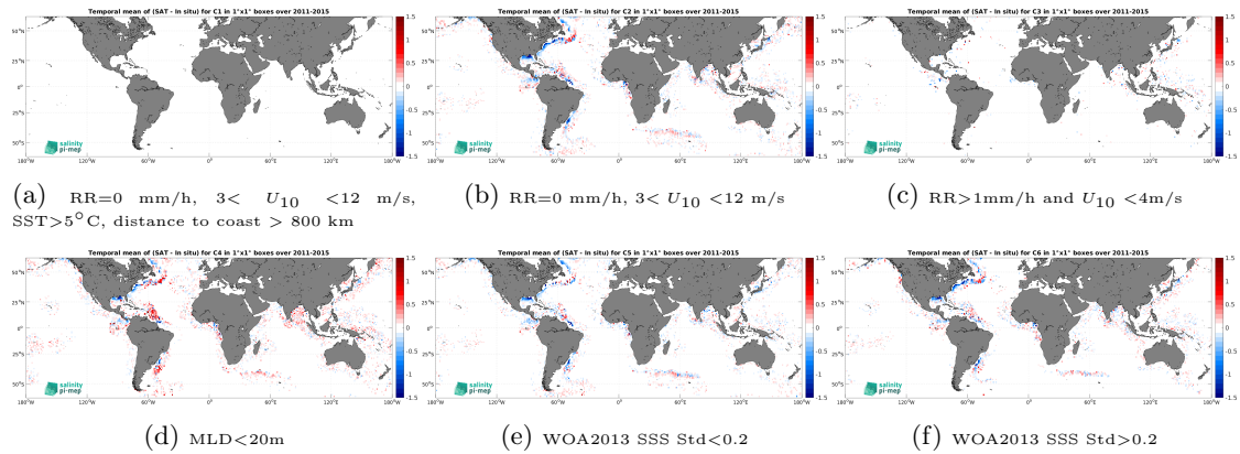
Figure 14: Temporal mean gridded over spatial boxes of size 1^\circ \times 1^\circ of \Delta SSS (Aquarius SSS L4 OI v5 - Weekly (IPRC) - Argo) for 6 different subdatasets corresponding to:RR=0 mm/h, 3 < U_{10} < 12 m/s, SST > 5^\circ\text{C} , distance to coast > 800 km (a), RR=0 mm/h, 3 < U_{10} < 12 m/s (b), RR > 1 mm/h and U_{10} < 4 m/s (c),MLD < 20 m (d),WOA2013 SSS Std < 0.2 (e),WOA2013 SSS Std > 0.2 (f).
