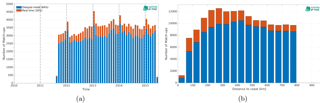
Figure 2: Number of match-ups between Argo and Aquarius SSS L4 OI v5 - Weekly (IPRC) SSS as a function of time (a) and as function of the distance to coast (b) over the SMOS coastal zone (<800km) 60N-60S Pi-MEP region and for the full satellite product period.
