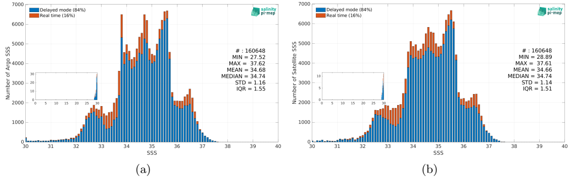
Figure 3: Histograms of SSS from Argo (a) and Aquarius SSS L4 OI v5 - Weekly (IPRC) (b) considering all match-up pairs per bins of 0.1 over the SMOS coastal zone (<800km) 60N-60S Pi-MEP region and for the full satellite product period.
