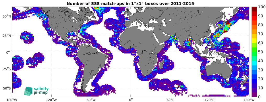
Figure 5: Number of SSS match-ups between Argo SSS and the Aquarius SSS L4 OI v5 - Weekly (IPRC) SSS product for the SMOS coastal zone (<800km) 60N-60S Pi-MEP region over 1^{\circ} \times 1^{\circ} boxes and for the full satellite product period.
