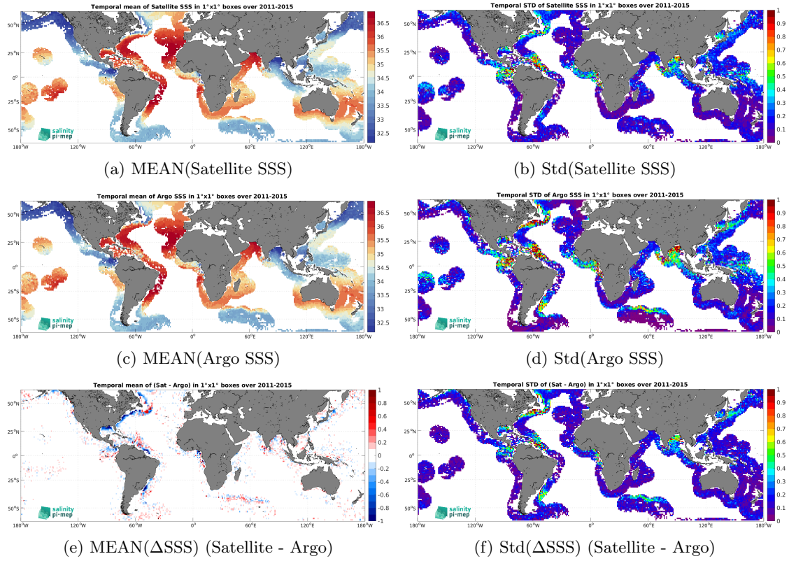
Figure 7: Temporal mean (left) and Std (right) of SSS from Aquarius SSS L4 OI v5 - Weekly (IPRC) (top), Argo (middle), and of \Delta SSS (Satellite - Argo). Only match-up pairs are used to generate these maps.
