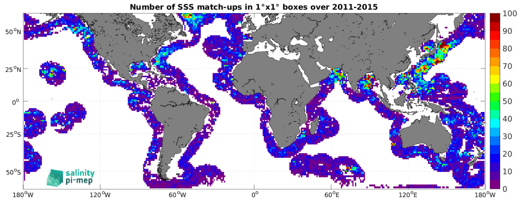
Figure 5: Number of SSS match-ups between Argo SSS and the Aquarius SSS L4 OI v5 - Weekly (IPRC) SSS product for the SMOS coastal zone (<800km) 60N-60S Pi-MEP region over 1^\circ \times 1^\circ boxes and for the full satellite product period.
