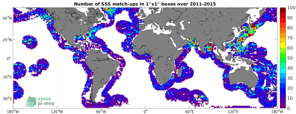
Figure 4: Number of SSS match-ups between Argo SSS and the Aquarius SSS L4 OI v5 - Weekly (IPRC) SSS product for the SMOS coastal zone (<800km) 60N-60S Pi-MEP region over 1^\circ \times 1^\circ boxes and for the full satellite product period.
