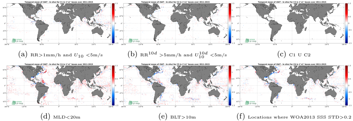
Figure 12: Temporal mean gridded over spatial boxes of size 1^\circ \times 1^\circ of \Delta SSS (Aquarius-L4-IPRC-V5-WEEKLY - Argo) for 6 different subdatasets corresponding to: RR > 1\text{mm/h} and U_{10} < 5\text{m/s} (a), RR^{10d} > 5\text{mm/h} and U_{10}^{10d} < 5\text{m/s} (b), C1 U C2 (c), MLD < 20\text{m} (d), BLT > 10\text{m} (e), Locations where WOA2013 SSS STD > 0.2 (f).
