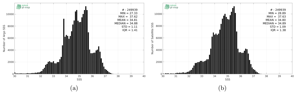
Figure 2: Histograms of SSS from Argo (a) and Aquarius-L4-IPRC-V5-WEEKLY (b) considering all match-up pairs per bins of 0.1 over the SMOS coastal zone ( \pm 800 km) 60N-60S Pi-MEP region and for the full satellite product period.
