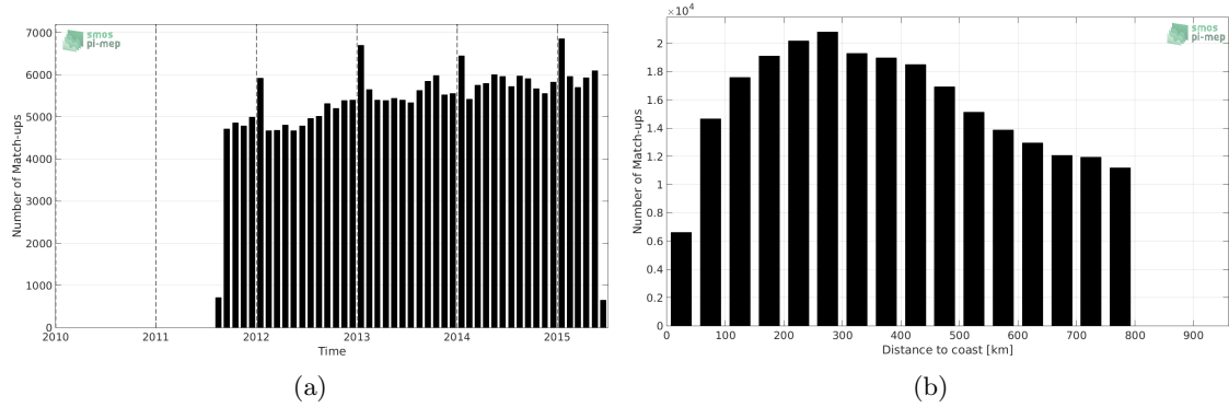
Figure 1: Number of match-ups between Argo and Aquarius-L4-IPRC-V5-WEEKLY SSS as a function of time (a) and as function of the distance to coast (b) over the SMOS coastal zone ( \pm 800 km) 60N-60S Pi-MEP region and for the full satellite product period.
