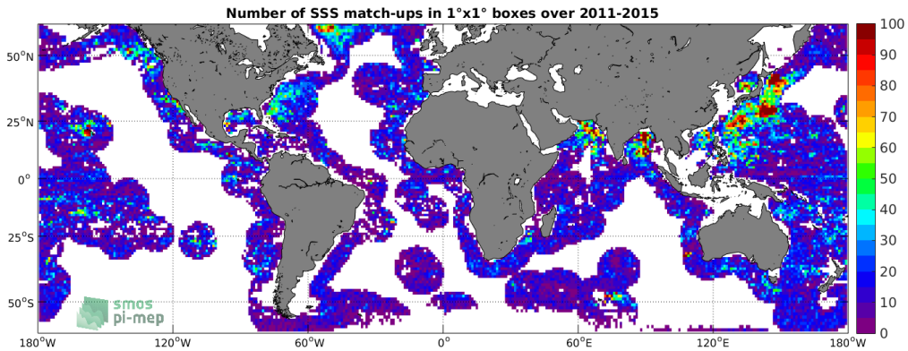
Figure 4: Number of SSS match-ups between Argo SSS and the Aquarius-L4-IPRC-V5-WEEKLY SSS product for the SMOS coastal zone ( \geq 800\text{km} ) 60N-60S Pi-MEP region over 1^\circ \times 1^\circ boxes and for the full satellite product period.
