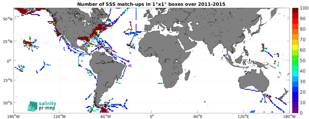
Figure 5: Number of SSS match-ups between TSG (SAMOS) SSS and the Aquarius SSS L4 OI v5 - Monthly (IPRC) SSS product for the SMOS coastal zone (<800km) 60N-60S Pi-MEP region over 1^{\circ} \times 1^{\circ} boxes and for the full satellite product period.
