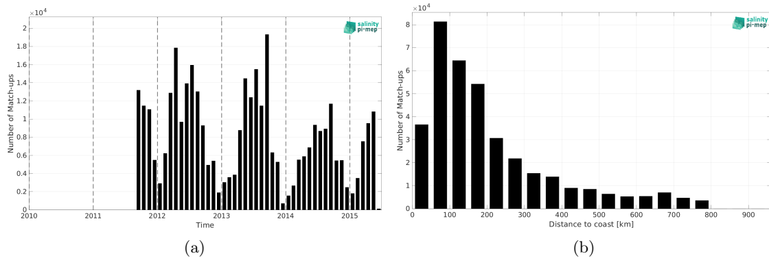
Figure 2: Number of match-ups between TSG (SAMOS) and Aquarius SSS L4 OI v5 - Monthly (IPRC) SSS as a function of time (a) and as function of the distance to coast (b) over the SMOS coastal zone (<800km) 60N-60S Pi-MEP region and for the full satellite product period.
