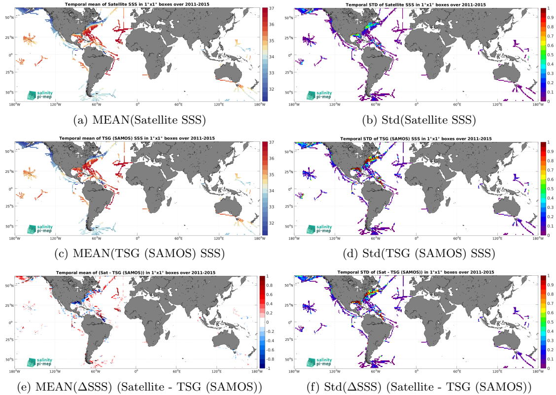
Figure 7: Temporal mean (left) and Std (right) of SSS from Aquarius SSS L4 OI v5 - Monthly (IPRC) (top), TSG (SAMOS) (middle), and of \Delta SSS (Satellite - TSG (SAMOS)). Only match-up pairs are used to generate these maps.
