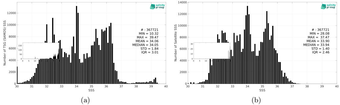
Figure 3: Histograms of SSS from TSG (SAMOS) (a) and Aquarius SSS L4 OI v5 - Monthly (IPRC) (b) considering all match-up pairs per bins of 0.1 over the SMOS coastal zone (<800km) 60N-60S Pi-MEP region and for the full satellite product period.
