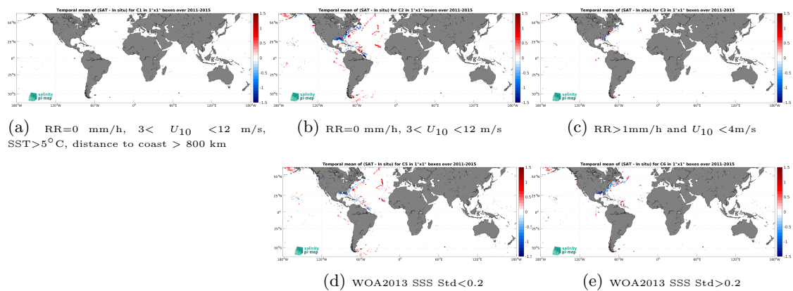
Figure 14: Temporal mean gridded over spatial boxes of size 1^\circ \times 1^\circ of \Delta SSS (Aquarius SSS L4 OI v5 - Monthly (IPRC) - TSG (SAMOS)) for 5 different subdatasets corresponding to:RR=0 mm/h, 3 < U_{10} < 12 m/s, SST >5^\circ\text{C} , distance to coast > 800 km (a), RR=0 mm/h, 3 < U_{10} < 12 m/s (b), RR >1 mm/h and U_{10} < 4 m/s (c), WOA2013 SSS Std <0.2 (d), WOA2013 SSS Std >0.2 (e).
