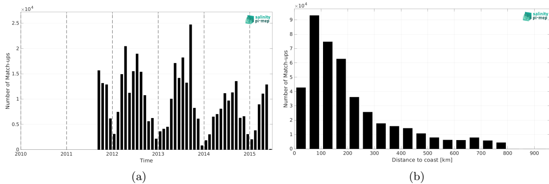
Figure 1: Number of match-ups between TSG (SAMOS) and Aquarius SSS L4 OI v5 - Monthly (IPRC) SSS as a function of time (a) and as function of the distance to coast (b) over the SMOS coastal zone ( < 800\text{km} ) 60N-60S Pi-MEP region and for the full satellite product period.
