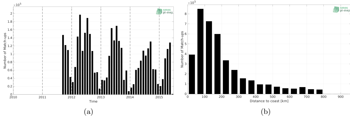
Figure 1: Number of match-ups between TSG (SAMOS) and Aquarius SSS L4 OI v5 - Monthly (IPRC) SSS as a function of time (a) and as function of the distance to coast (b) over the SMOS coastal zone (<800km) 60N-60S Pi-MEP region and for the full satellite product period.
