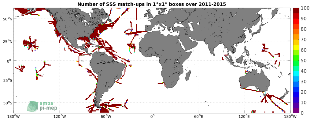
Figure 4: Number of SSS match-ups between TSG (SAMOS) SSS and the Aquarius SSS L4 OI v5 - Monthly (IPRC) SSS product for the SMOS coastal zone (<800km) 60N-60S Pi-MEP region over 1^\circ \times 1^\circ boxes and for the full satellite product period.
