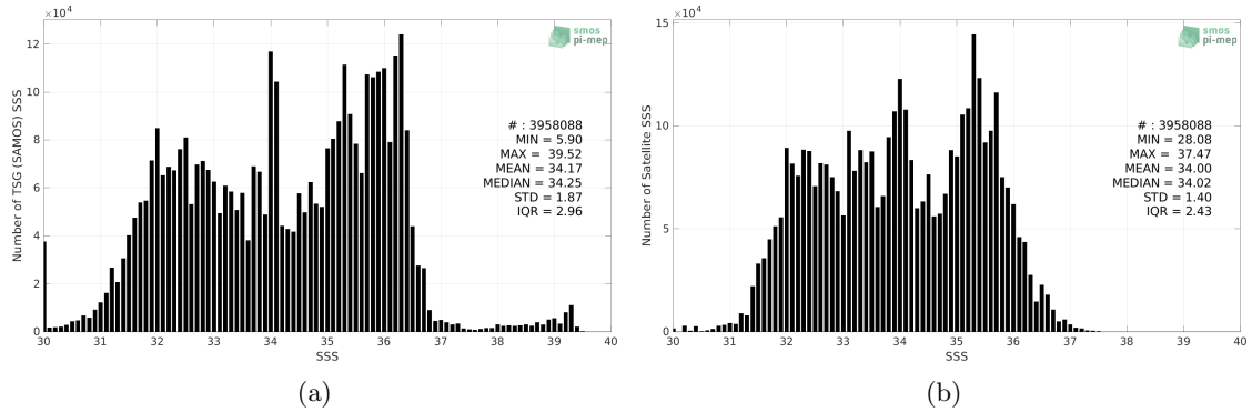
Figure 2: Histograms of SSS from TSG (SAMOS) (a) and Aquarius SSS L4 OI v5 - Monthly (IPRC) (b) considering all match-up pairs per bins of 0.1 over the SMOS coastal zone (<800km) 60N-60S Pi-MEP region and for the full satellite product period.
