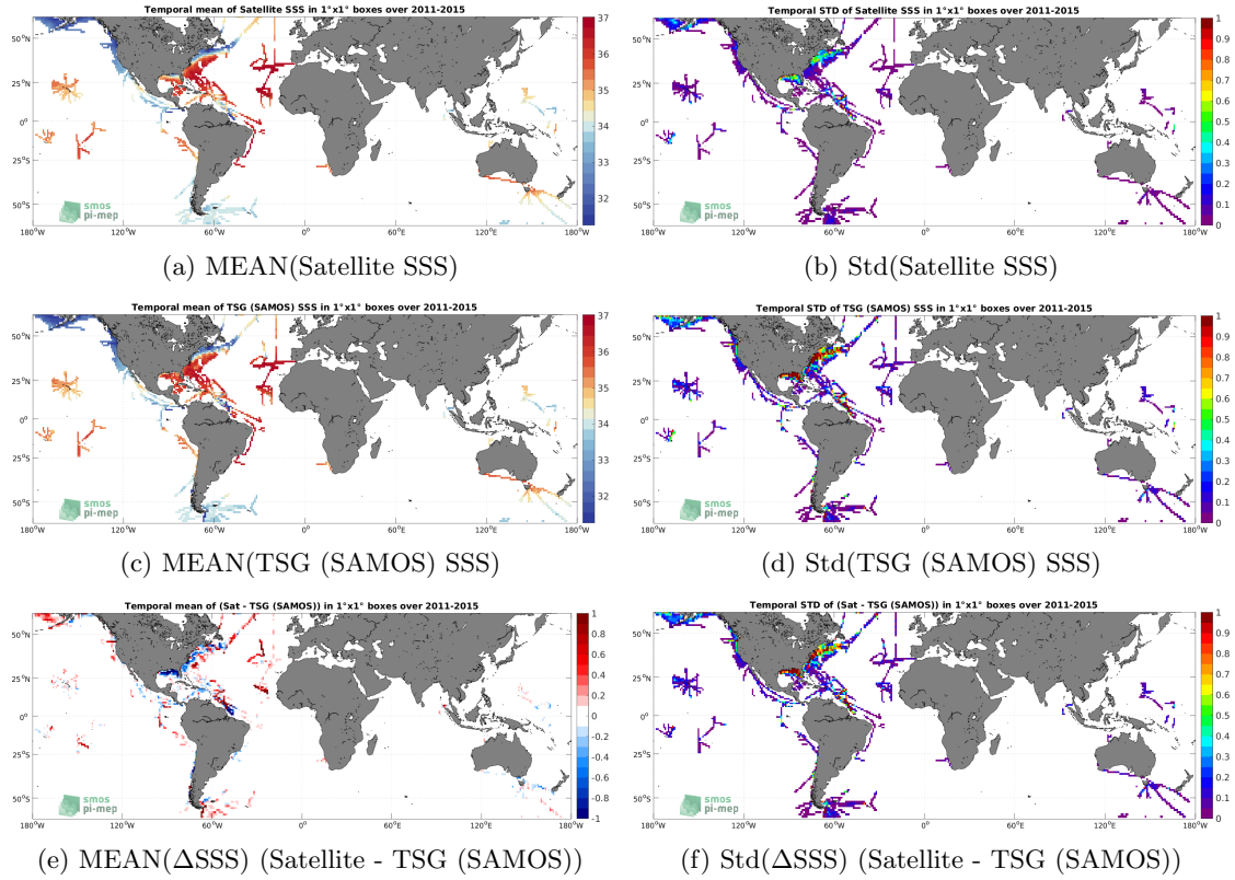
Figure 6: Temporal mean (left) and Std (right) of SSS from Aquarius SSS L4 OI v5 - Monthly (IPRC) (top), TSG (SAMOS) (middle), and of \Delta SSS (Satellite - TSG (SAMOS)). Only match-up pairs are used to generate these maps.
