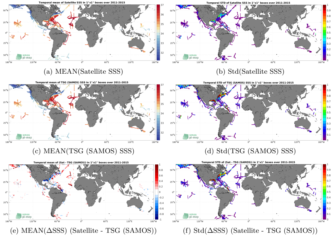
Figure 6: Temporal mean (left) and Std (right) of SSS from Aquarius SSS L4 OI v5 - Monthly (IPRC) (top), TSG (SAMOS) in situ dataset (middle), and of \Delta SSS (Satellite - TSG (SAMOS)). Only match-up pairs are used to generate these maps.
