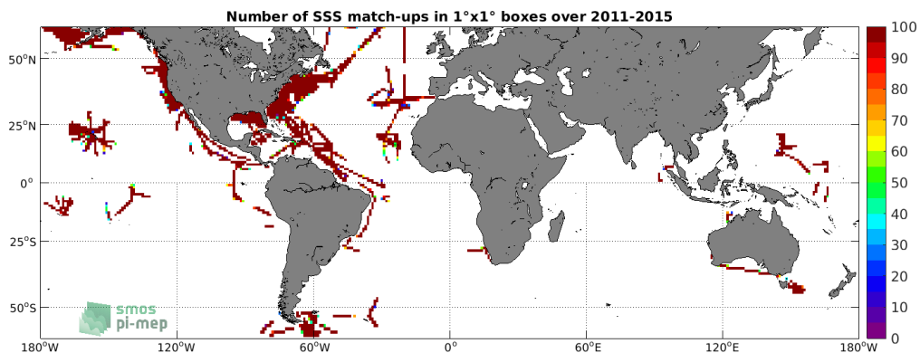
Figure 4: Number of SSS match-ups between TSG (SAMOS) SSS and the Aquarius SSS L4 OI v5 - Monthly (IPRC) SSS product for the SMOS coastal zone (<800km) 60N-60S Pi-MEP region over 1°x1° boxes and for the full satellite product period.
