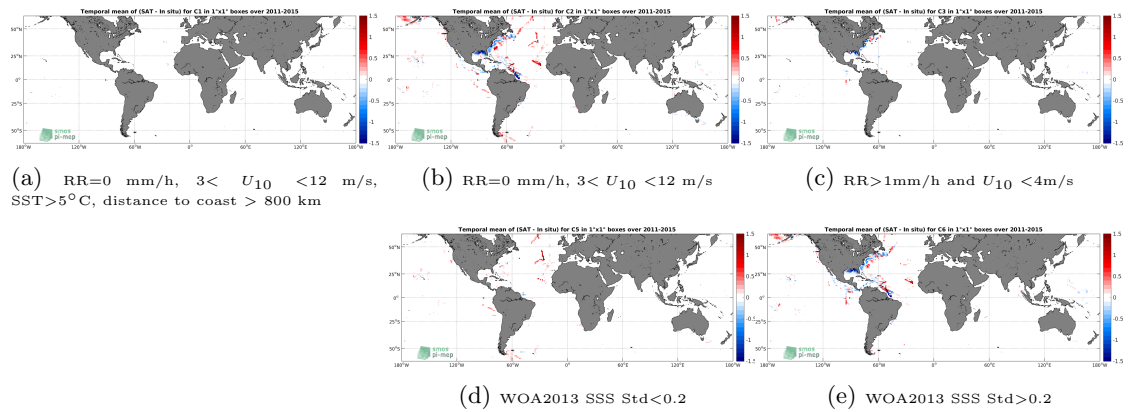
Figure 12: Temporal mean gridded over spatial boxes of size 1^\circ \times 1^\circ of \Delta SSS (Aquarius-L4-IPRC-V5-MONTHLY - TSG-SAMOS) for 5 different subdatasets corresponding to:RR=0 mm/h, 3 < U_{10} < 12 m/s, SST >5^\circ C, distance to coast > 800 km (a), RR=0 mm/h, 3 < U_{10} < 12 m/s (b), RR >1 mm/h and U_{10} < 4 m/s (c), WOA2013 SSS Std <0.2 (d), WOA2013 SSS Std >0.2 (e).
