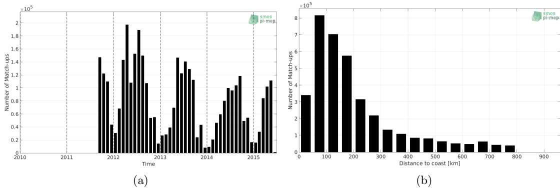
Figure 1: Number of match-ups between TSG-SAMOS and Aquarius-L4-IPRC-V5-MONTHLY SSS as a function of time (a) and as function of the distance to coast (b) over the SMOS coastal zone (<800km) 60N-60S Pi-MEP region and for the full satellite product period.
