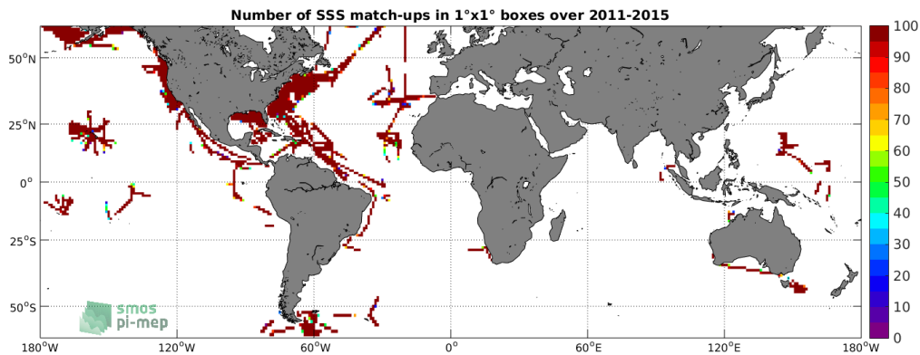
Figure 4: Number of SSS match-ups between TSG-SAMOS SSS and the Aquarius-L4-IPRC-V5-MONTHLY SSS product for the SMOS coastal zone (<800km) 60N-60S Pi-MEP region over 1°x1° boxes and for the full satellite product period.
