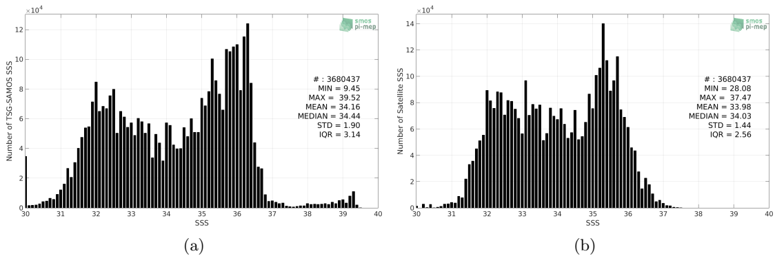
Figure 2: Histograms of SSS from TSG-SAMOS (a) and Aquarius-L4-IPRC-V5-MONTHLY (b) considering all match-up pairs per bins of 0.1 over the SMOS coastal zone (<800km) 60N-60S Pi-MEP region and for the full satellite product period.
