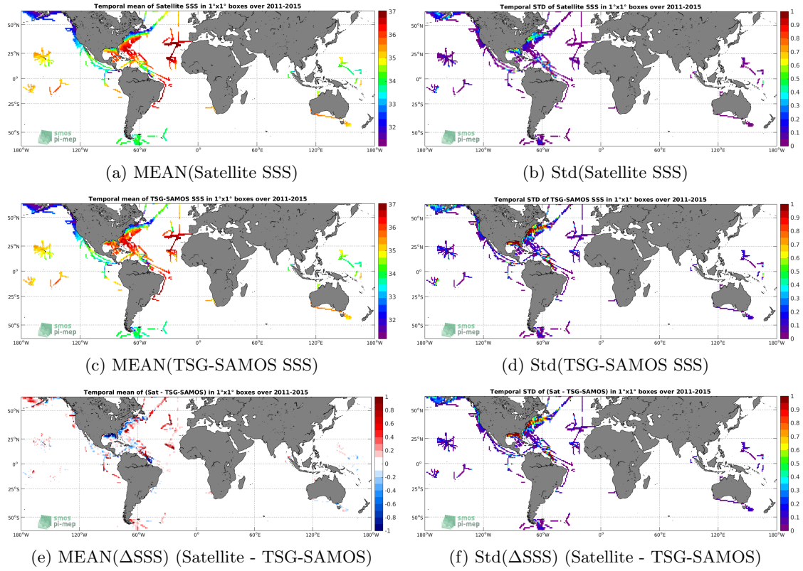
Figure 6: Temporal mean (left) and Std (right) of SSS from Aquarius-L4-IPRC-V5-MONTHLY (top), TSG-SAMOS (middle), and of \Delta SSS (Satellite - TSG-SAMOS). Only match-up pairs are used to generate these maps.
