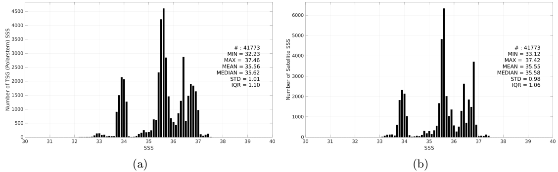
Figure 3: Histograms of SSS from TSG (Polarstern) (a) and Aquarius SSS L4 OI v5 - Monthly (IPRC) (b) considering all match-up pairs per bins of 0.1 over the SMOS coastal zone (<800km) 60N-60S Pi-MEP region and for the full satellite product period.
