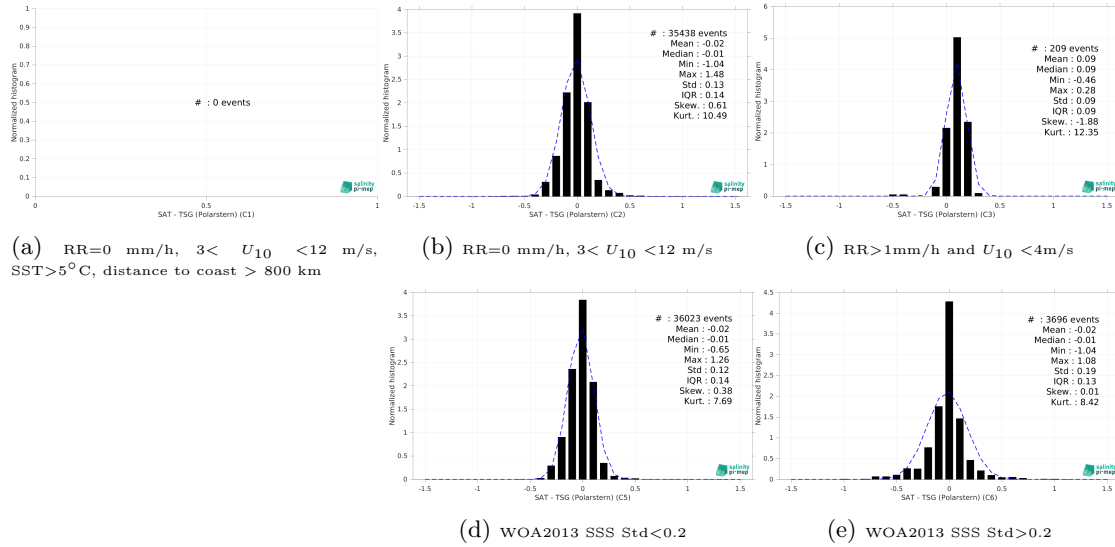
Figure 15: Normalized histogram of \Delta SSS (Aquarius SSS L4 OI v5 - Monthly (IPRC) - TSG (Polarstern)) for 5 different subdatasets corresponding to: RR=0 mm/h, 3 < U_{10} < 12 m/s, SST > 5°C, distance to coast > 800 km (a), RR=0 mm/h, 3 < U_{10} < 12 m/s (b), RR > 1mm/h and U_{10} < 4 m/s (c), WOA2013 SSS Std < 0.2 (d), WOA2013 SSS Std > 0.2 (e).
