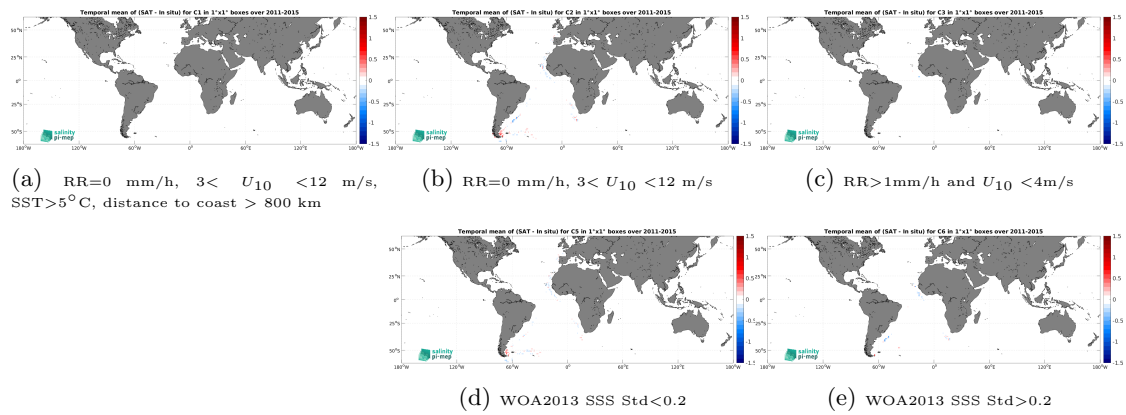
Figure 14: Temporal mean gridded over spatial boxes of size 1^\circ \times 1^\circ of \Delta SSS (Aquarius SSS L4 OI v5 - Monthly (IPRC) - TSG (Polarstern)) for 5 different subdatasets corresponding to:RR=0 mm/h, 3 < U_{10} < 12 m/s, SST >5^\circ\text{C} , distance to coast > 800 km (a), RR=0 mm/h, 3 < U_{10} < 12 m/s (b), RR >1 mm/h and U_{10} < 4 m/s (c), WOA2013 SSS Std <0.2 (d), WOA2013 SSS Std >0.2 (e).
