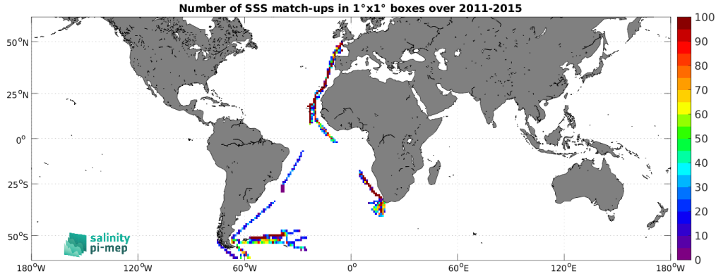
Figure 5: Number of SSS match-ups between TSG (Polarstern) SSS and the Aquarius SSS L4 OI v5 - Monthly (IPRC) SSS product for the SMOS coastal zone (<800km) 60N-60S Pi-MEP region over 1^{\circ} \times 1^{\circ} boxes and for the full satellite product period.
