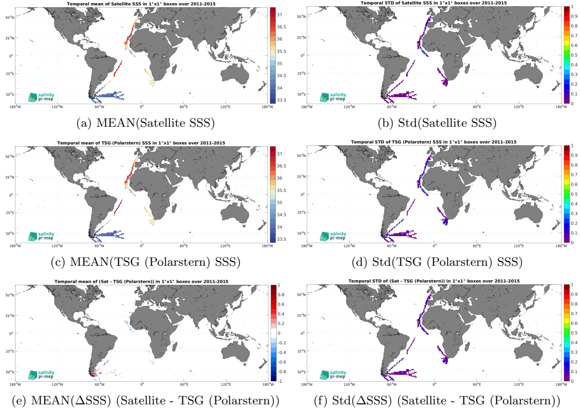
Figure 7: Temporal mean (left) and Std (right) of SSS from Aquarius SSS L4 OI v5 - Monthly (IPRC) (top), TSG (Polarstern) (middle), and of \Delta SSS (Satellite - TSG (Polarstern)). Only match-up pairs are used to generate these maps.
