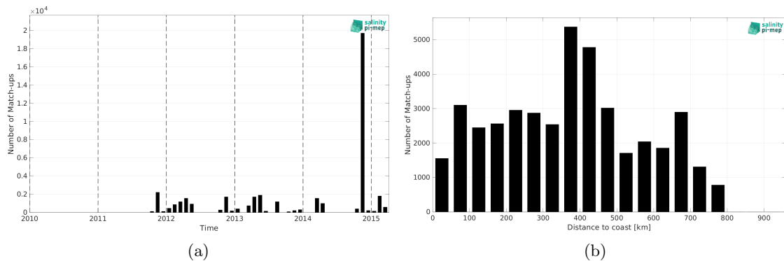
Figure 2: Number of match-ups between TSG (Polarstern) and Aquarius SSS L4 OI v5 - Monthly (IPRC) SSS as a function of time (a) and as function of the distance to coast (b) over the SMOS coastal zone (<800km) 60N-60S Pi-MEP region and for the full satellite product period.
