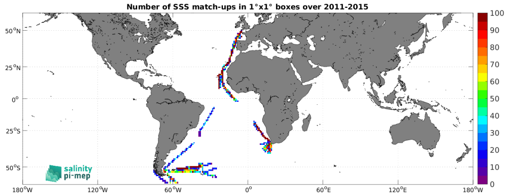
Figure 4: Number of SSS match-ups between TSG (Polarstern) SSS and the Aquarius SSS L4 OI v5 - Monthly (IPRC) SSS product for the SMOS coastal zone (<800km) 60N-60S Pi-MEP region over 1^{\circ} \times 1^{\circ} boxes and for the full satellite product period.
