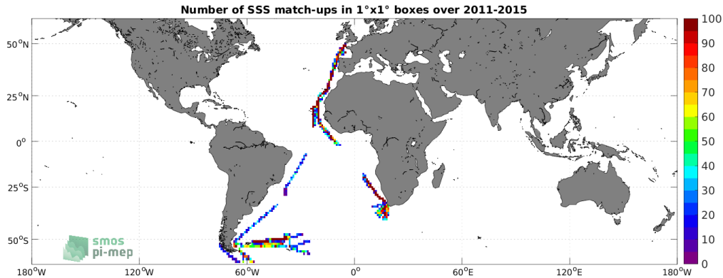
Figure 4: Number of SSS match-ups between TSG (Polarstern) SSS and the Aquarius SSS L4 OI v5 - Monthly (IPRC) SSS product for the SMOS coastal zone (<800km) 60N-60S Pi-MEP region over 1^\circ \times 1^\circ boxes and for the full satellite product period.
