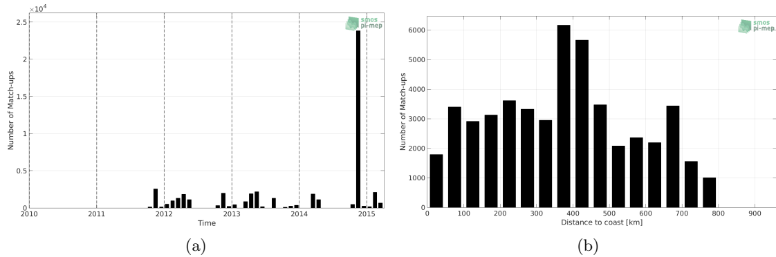
Figure 1: Number of match-ups between TSG-POLARSTERN and Aquarius-L4-IPRC-V5-MONTHLY SSS as a function of time (a) and as function of the distance to coast (b) over the SMOS coastal zone ( \pm 800 km) 60N-60S Pi-MEP region and for the full satellite product period.
