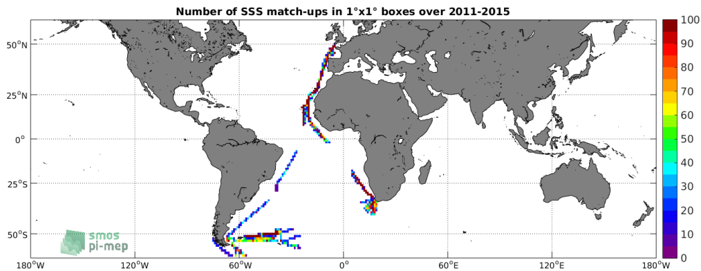
Figure 4: Number of SSS match-ups between TSG-POLARSTERN SSS and the Aquarius-L4-IPRC-V5-MONTHLY SSS product for the SMOS coastal zone ( \pm 800\text{km} ) 60N-60S Pi-MEP region over 1^\circ \times 1^\circ boxes and for the full satellite product period.
