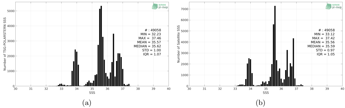
Figure 2: Histograms of SSS from TSG-POLARSTERN (a) and Aquarius-L4-IPRC-V5-MONTHLY (b) considering all match-up pairs per bins of 0.1 over the SMOS coastal zone ( \pm 800 km) 60N-60S Pi-MEP region and for the full satellite product period.
