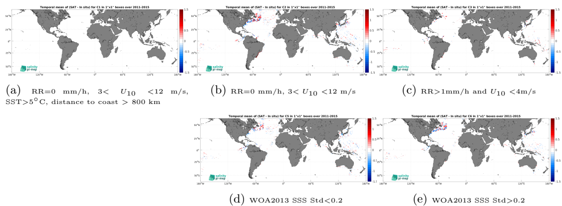
Figure 14: Temporal mean gridded over spatial boxes of size 1^\circ \times 1^\circ of \Delta SSS (Aquarius SSS L4 OI v5 - Monthly (IPRC) - TSG (LEGOS-DM)) for 5 different subdatasets corresponding to:RR=0 mm/h, 3 < U_{10} < 12 m/s, SST >5^\circ\text{C} , distance to coast > 800 km (a), RR=0 mm/h, 3 < U_{10} < 12 m/s (b), RR >1 mm/h and U_{10} < 4 m/s (c), WOA2013 SSS Std <0.2 (d), WOA2013 SSS Std >0.2 (e).
