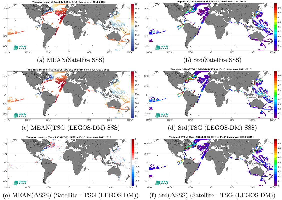
Figure 7: Temporal mean (left) and Std (right) of SSS from Aquarius SSS L4 OI v5 - Monthly (IPRC) (top), TSG (LEGOS-DM) (middle), and of \Delta SSS (Satellite - TSG (LEGOS-DM)). Only match-up pairs are used to generate these maps.
