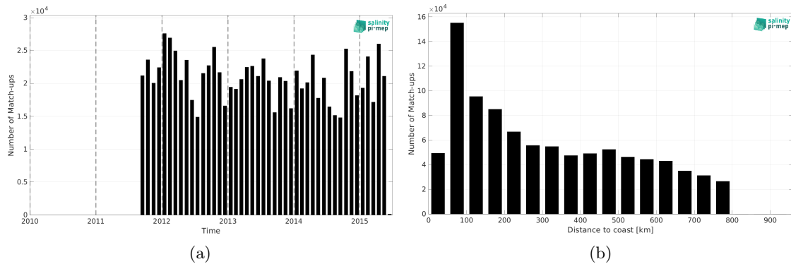
Figure 2: Number of match-ups between TSG (LEGOS-DM) and Aquarius SSS L4 OI v5 - Monthly (IPRC) SSS as a function of time (a) and as function of the distance to coast (b) over the SMOS coastal zone (<800km) 60N-60S Pi-MEP region and for the full satellite product period.
