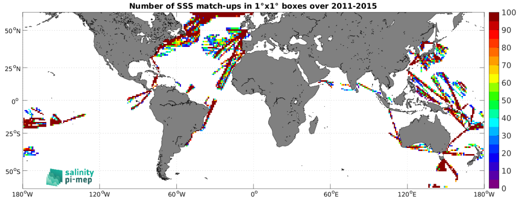
Figure 5: Number of SSS match-ups between TSG (LEGOS-DM) SSS and the Aquarius SSS L4 OI v5 - Monthly (IPRC) SSS product for the SMOS coastal zone (<800km) 60N-60S Pi-MEP region over 1^{\circ} \times 1^{\circ} boxes and for the full satellite product period.
