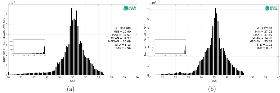
Figure 3: Histograms of SSS from TSG (LEGOS-DM) (a) and Aquarius SSS L4 OI v5 - Monthly (IPRC) (b) considering all match-up pairs per bins of 0.1 over the SMOS coastal zone (<800km) 60N-60S Pi-MEP region and for the full satellite product period.
