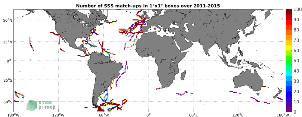
Figure 4: Number of SSS match-ups between TSG-GOSUD-Sailing-ship SSS and the Aquarius-L4-IPRC-V5-MONTHLY SSS product for the SMOS coastal zone (<800km) 60N-60S Pi-MEP region over 1°x1° boxes and for the full satellite product period.
