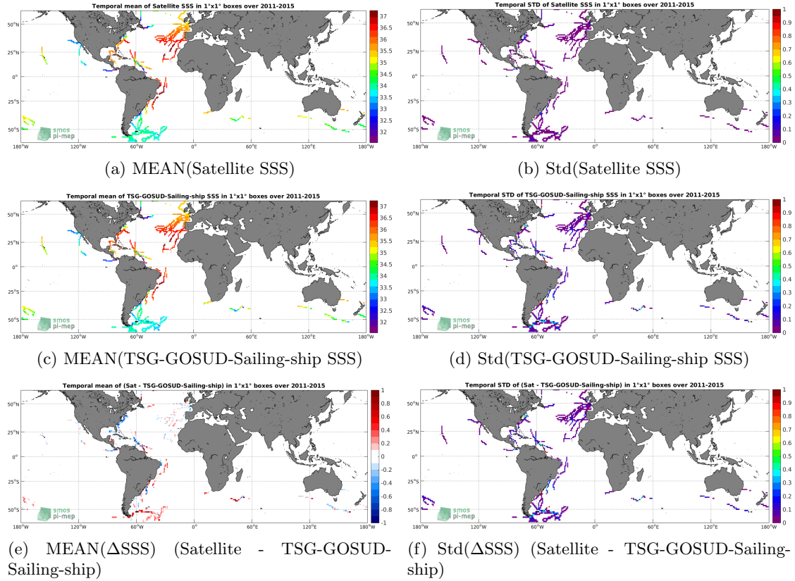
Figure 6: Temporal mean (left) and Std (right) of SSS from Aquarius-L4-IPRC-V5-MONTHLY (top), TSG-GOSUD-Sailing-ship (middle), and of \Delta SSS (Satellite - TSG-GOSUD-Sailing-ship). Only match-up pairs are used to generate these maps.
