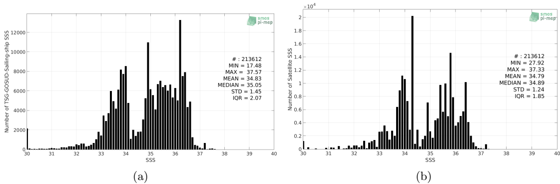
Figure 2: Histograms of SSS from TSG-GOSUD-Sailing-ship (a) and Aquarius-L4-IPRC-V5-MONTHLY (b) considering all match-up pairs per bins of 0.1 over the SMOS coastal zone (<800km) 60N-60S Pi-MEP region and for the full satellite product period.
