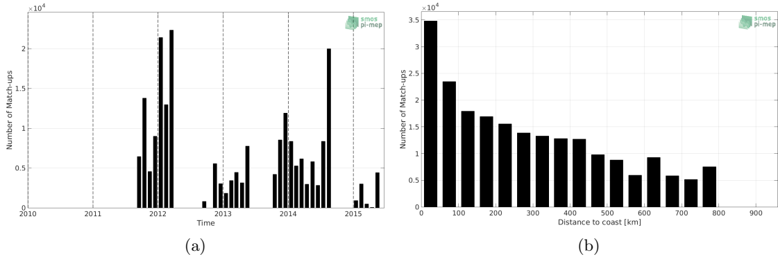
Figure 1: Number of match-ups between TSG-GOSUD-Sailing-ship and Aquarius-L4-IPRC-V5-MONTHLY SSS as a function of time (a) and as function of the distance to coast (b) over the SMOS coastal zone (<800km) 60N-60S Pi-MEP region and for the full satellite product period.
