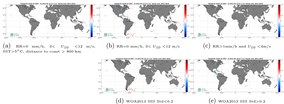
Figure 12: Temporal mean gridded over spatial boxes of size 1^\circ \times 1^\circ of \Delta SSS (Aquarius-L4-IPRC-V5-MONTHLY - TSG-GOSUD-Sailing-ship) for 5 different subdatasets corresponding to: RR=0 mm/h, 3 < U_{10} < 12 m/s, SST > 5°C, distance to coast > 800 km (a), RR=0 mm/h, 3 < U_{10} < 12 m/s (b), RR > 1mm/h and U_{10} < 4 m/s (c), WOA2013 SSS Std < 0.2 (d), WOA2013 SSS Std > 0.2 (e).
