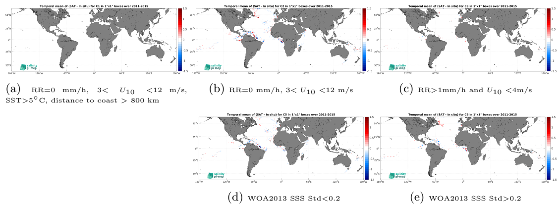
Figure 14: Temporal mean gridded over spatial boxes of size 1^\circ \times 1^\circ of \Delta\text{SSS} (Aquarius SSS L4 OI v5 - Monthly (IPRC) - TSG (GOSUD-Research-vessel)) for 5 different subdatasets corresponding to: RR=0 mm/h, 3 < U_{10} < 12 m/s, SST > 5°C, distance to coast > 800 km (a), RR=0 mm/h, 3 < U_{10} < 12 m/s (b), RR > 1mm/h and U_{10} < 4 m/s (c), WOA2013 SSS Std < 0.2 (d), WOA2013 SSS Std > 0.2 (e).
