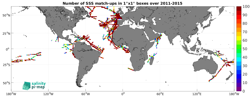
Figure 5: Number of SSS match-ups between TSG (GOSUD-Research-vessel) SSS and the Aquarius SSS L4 OI v5 - Monthly (IPRC) SSS product for the SMOS coastal zone (<800km) 60N-60S Pi-MEP region over 1^\circ \times 1^\circ boxes and for the full satellite product period.
