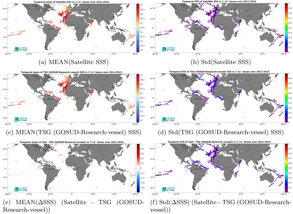
Figure 7: Temporal mean (left) and Std (right) of SSS from Aquarius SSS L4 OI v5 - Monthly (IPRC) (top), TSG (GOSUD-Research-vessel) (middle), and of \Delta SSS (Satellite - TSG (GOSUD-Research-vessel)). Only match-up pairs are used to generate these maps.
