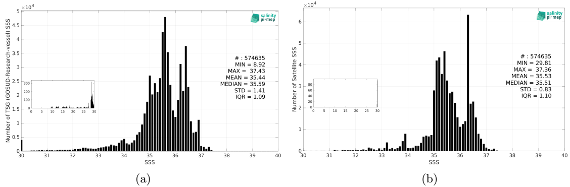
Figure 3: Histograms of SSS from TSG (GOSUD-Research-vessel) (a) and Aquarius SSS L4 OI v5 - Monthly (IPRC) (b) considering all match-up pairs per bins of 0.1 over the SMOS coastal zone (<800km) 60N-60S Pi-MEP region and for the full satellite product period.
