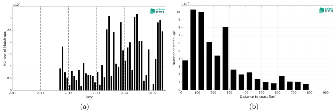
Figure 2: Number of match-ups between TSG (GOSUD-Research-vessel) and Aquarius SSS L4 OI v5 - Monthly (IPRC) SSS as a function of time (a) and as function of the distance to coast (b) over the SMOS coastal zone (<800km) 60N-60S Pi-MEP region and for the full satellite product period.
