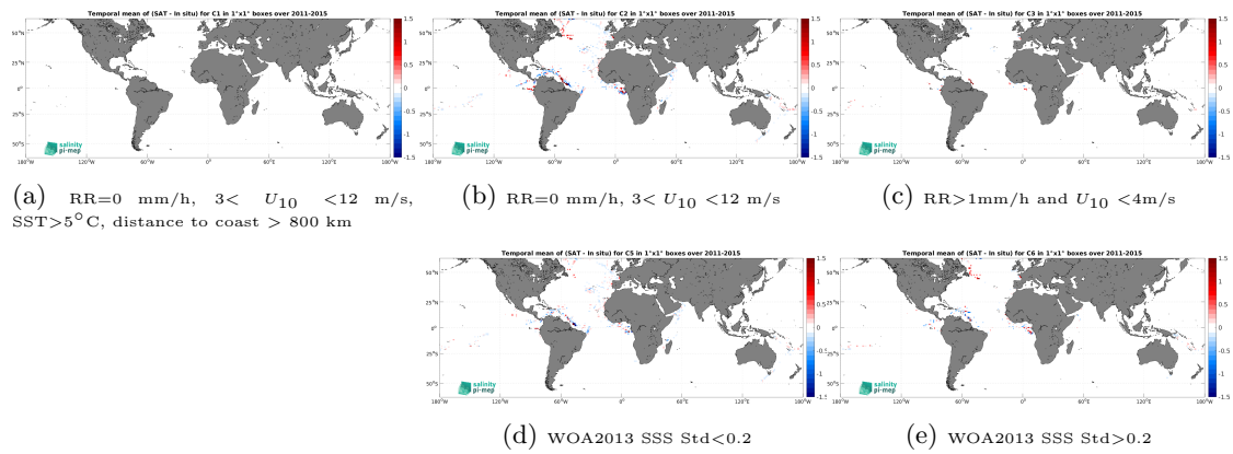
Figure 12: Temporal mean gridded over spatial boxes of size 1^\circ \times 1^\circ of \Delta\text{SSS} (Aquarius SSS L4 OI v5 - Monthly (IPRC) - TSG (GOSUD-Research-vessel)) for 5 different subdatasets corresponding to:RR=0 mm/h, 3 < U_{10} < 12 m/s, SST >5^\circ\text{C} , distance to coast > 800 km (a), RR=0 mm/h, 3 < U_{10} < 12 m/s (b), RR >1 mm/h and U_{10} < 4 m/s (c), WOA2013 SSS Std <0.2 (d), WOA2013 SSS Std >0.2 (e).
