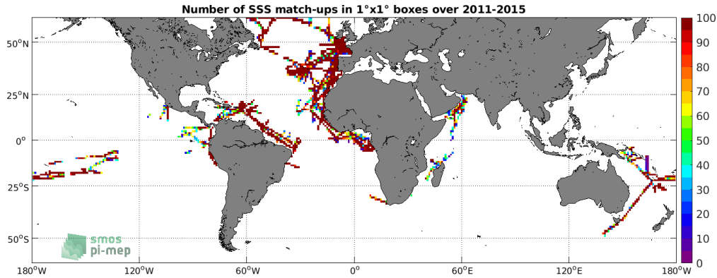
Figure 4: Number of SSS match-ups between TSG (GOSUD-Research-vessel) SSS and the Aquarius SSS L4 OI v5 - Monthly (IPRC) SSS product for the SMOS coastal zone (<800km) 60N-60S Pi-MEP region over 1^{\circ} \times 1^{\circ} boxes and for the full satellite product period.
