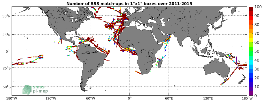
Figure 4: Number of SSS match-ups between TSG (GOSUD-Research-vessel) SSS and the Aquarius SSS L4 OI v5 - Monthly (IPRC) SSS product for the SMOS coastal zone (<800km) 60N-60S Pi-MEP region over 1°x1° boxes and for the full satellite product period.
