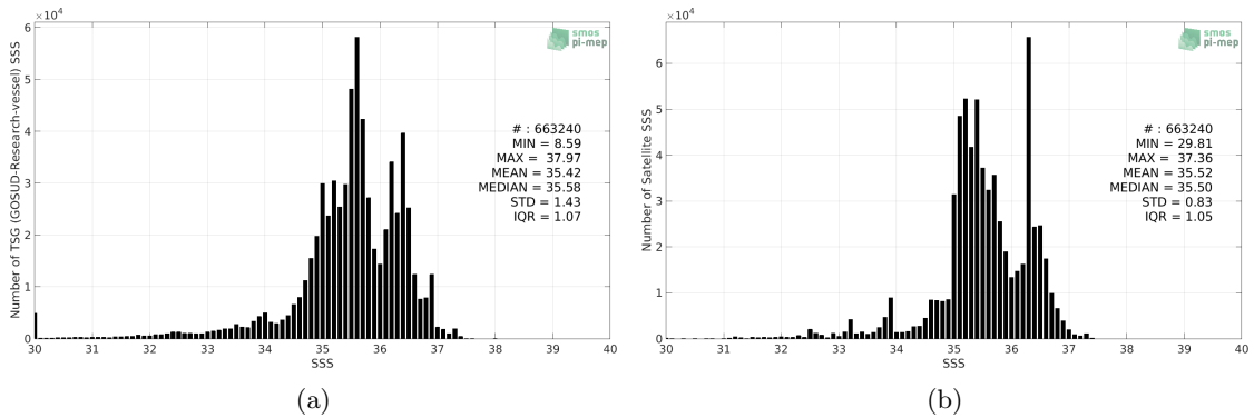
Figure 2: Histograms of SSS from TSG (GOSUD-Research-vessel) (a) and Aquarius SSS L4 OI v5 - Monthly (IPRC) (b) considering all match-up pairs per bins of 0.1 over the SMOS coastal zone (<800km) 60N-60S Pi-MEP region and for the full satellite product period.
