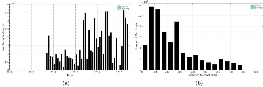
Figure 1: Number of match-ups between TSG (GOSUD-Research-vessel) and Aquarius SSS L4 OI v5 - Monthly (IPRC) SSS as a function of time (a) and as function of the distance to coast (b) over the SMOS coastal zone (<800km) 60N-60S Pi-MEP region and for the full satellite product period.
