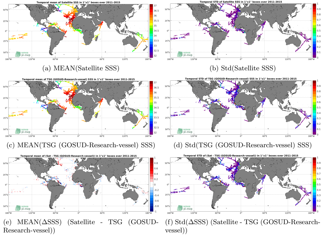
Figure 6: Temporal mean (left) and Std (right) of SSS from Aquarius SSS L4 OI v5 - Monthly (IPRC) (top), TSG (GOSUD-Research-vessel) (middle), and of \Delta SSS (Satellite - TSG (GOSUD-Research-vessel)). Only match-up pairs are used to generate these maps.
