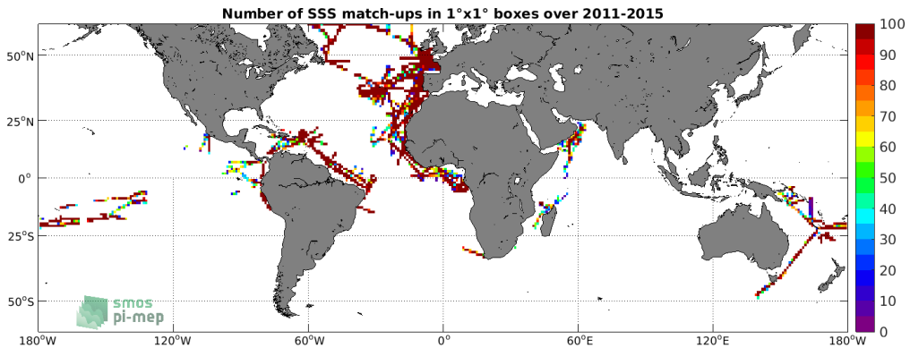
Figure 4: Number of SSS match-ups between TSG (GOSUD-Research-vessel) SSS and the Aquarius SSS L4 OI v5 - Monthly (IPRC) SSS product for the SMOS coastal zone (<800km) 60N-60S Pi-MEP region over 1^\circ \times 1^\circ boxes and for the full satellite product period.
