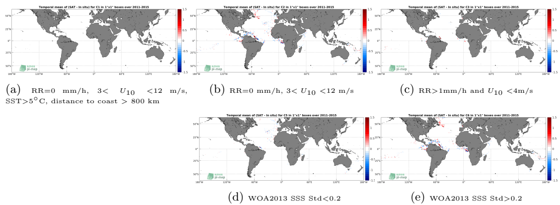
Figure 12: Temporal mean gridded over spatial boxes of size 1^\circ \times 1^\circ of \Delta SSS (Aquarius SSS L4 OI v5 - Monthly (IPRC) - TSG (GOSUD-Research-vessel)) for 5 different subdatasets corresponding to: RR=0 mm/h, 3 < U_{10} < 12 m/s, SST > 5°C, distance to coast > 800 km (a), RR=0 mm/h, 3 < U_{10} < 12 m/s (b), RR > 1mm/h and U_{10} < 4 m/s (c), WOA2013 SSS Std < 0.2 (d), WOA2013 SSS Std > 0.2 (e).
