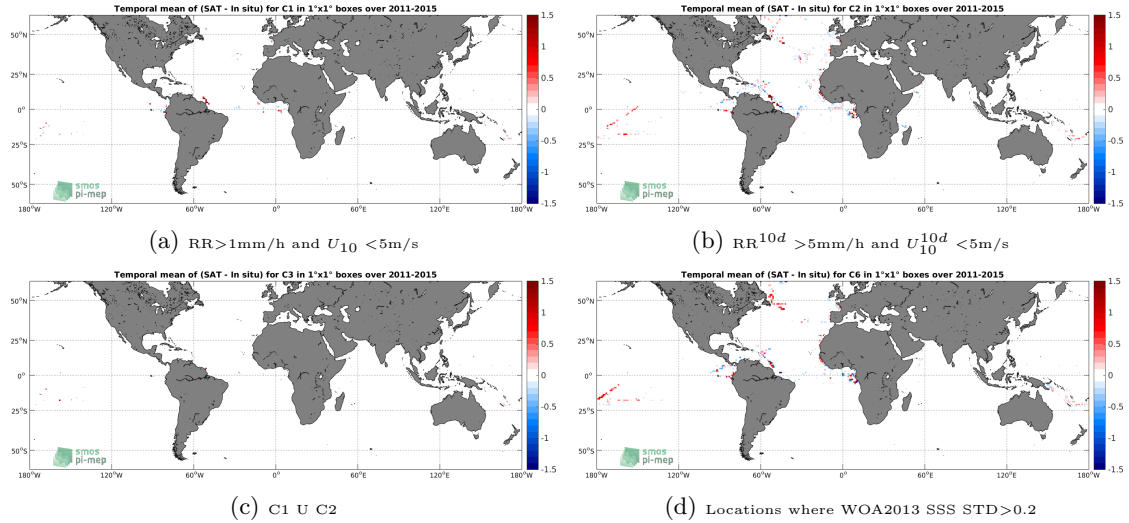
Figure 12: Temporal mean gridded over spatial boxes of size 1^\circ \times 1^\circ of \Delta SSS (Aquarius-L4-IPRC-V5-MONTHLY - TSG-GOSUD-Research-vessel) for 4 different subdatasets corresponding to: RR > 1\text{mm/h} and U_{10} < 5\text{m/s} (a), RR^{10d} > 5\text{mm/h} and U_{10}^{10d} < 5\text{m/s} (b), C1 U C2 (c), Locations where WOA2013 SSS STD > 0.2 (d).
