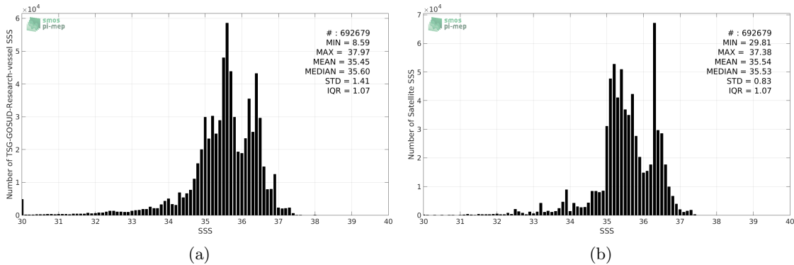
Figure 2: Histograms of SSS from TSG-GOSUD-Research-vessel (a) and Aquarius-L4-IPRC-V5-MONTHLY (b) considering all match-up pairs per bins of 0.1 over the SMOS coastal zone ( \approx 800 km) 60N-60S Pi-MEP region and for the full satellite product period.
