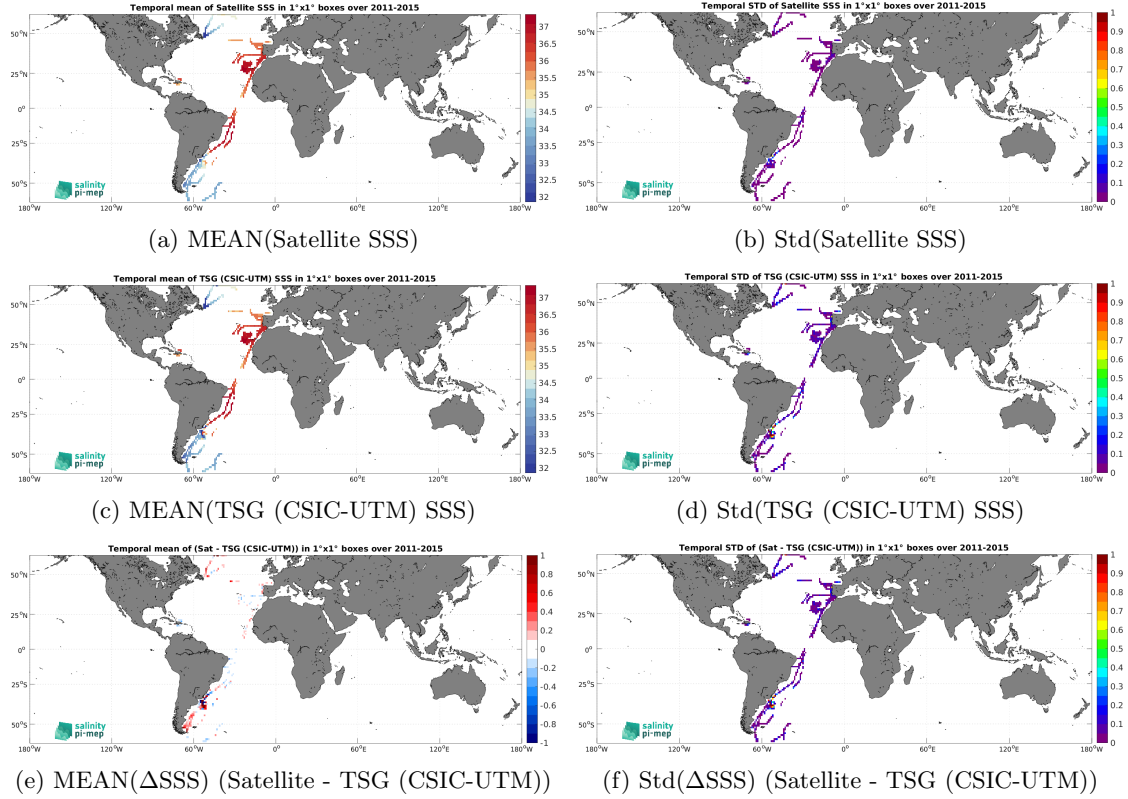
Figure 7: Temporal mean (left) and Std (right) of SSS from Aquarius SSS L4 OI v5 - Monthly (IPRC) (top), TSG (CSIC-UTM) (middle), and of \Delta SSS (Satellite - TSG (CSIC-UTM)). Only match-up pairs are used to generate these maps.
