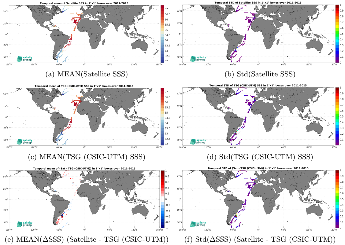
Figure 6: Temporal mean (left) and Std (right) of SSS from Aquarius SSS L4 OI v5 - Monthly (IPRC) (top), TSG (CSIC-UTM) (middle), and of \Delta SSS (Satellite - TSG (CSIC-UTM)). Only match-up pairs are used to generate these maps.
