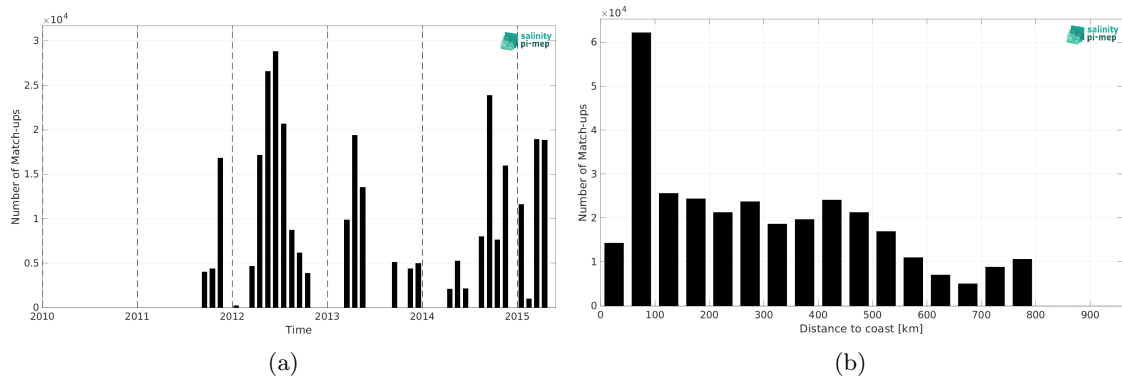
Figure 1: Number of match-ups between TSG (CSIC-UTM) and Aquarius SSS L4 OI v5 - Monthly (IPRC) SSS as a function of time (a) and as function of the distance to coast (b) over the SMOS coastal zone (<800km) 60N-60S Pi-MEP region and for the full satellite product period.
