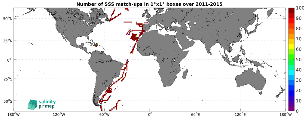
Figure 4: Number of SSS match-ups between TSG (CSIC-UTM) SSS and the Aquarius SSS L4 OI v5 - Monthly (IPRC) SSS product for the SMOS coastal zone (<800km) 60N-60S Pi-MEP region over 1^{\circ} \times 1^{\circ} boxes and for the full satellite product period.
