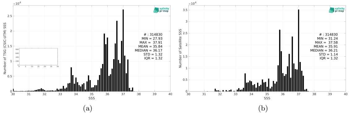
Figure 2: Histograms of SSS from TSG (CSIC-UTM) (a) and Aquarius SSS L4 OI v5 - Monthly (IPRC) (b) considering all match-up pairs per bins of 0.1 over the SMOS coastal zone (<800km) 60N-60S Pi-MEP region and for the full satellite product period.
