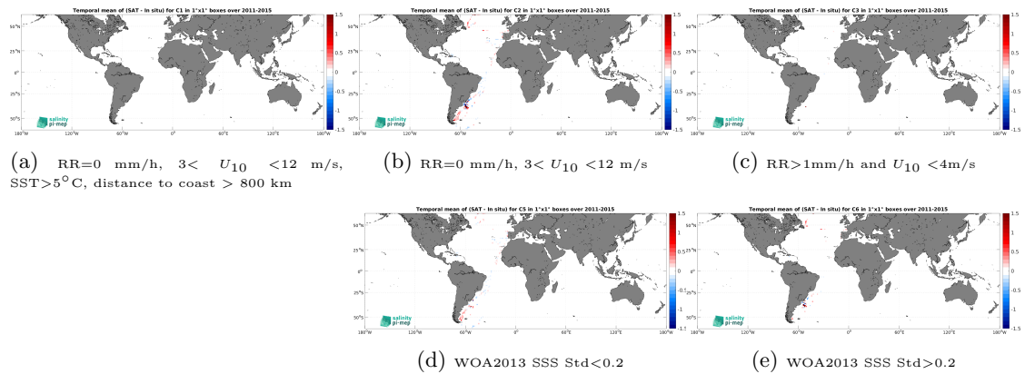
Figure 12: Temporal mean gridded over spatial boxes of size 1^\circ \times 1^\circ of \Delta\text{SSS} (Aquarius SSS L4 OI v5 - Monthly (IPRC) - TSG (CSIC-UTM)) for 5 different subdatasets corresponding to:RR=0 mm/h, 3 < U_{10} < 12 m/s, SST >5^\circ\text{C} , distance to coast > 800 km (a), RR=0 mm/h, 3 < U_{10} < 12 m/s (b), RR >1 mm/h and U_{10} < 4 m/s (c), WOA2013 SSS Std <0.2 (d), WOA2013 SSS Std >0.2 (e).
