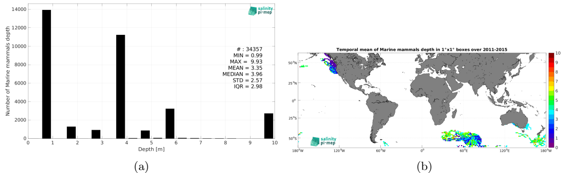
Figure 4: Histograms of the depth of the upper level SSS measurements from Marine mammals in the Match-up DataBase for the SMOS coastal zone (<800km) 60N-60S Pi-MEP region (a) and temporal mean spatial distribution of pressure of the in situ SSS data over 1^\circ \times 1^\circ boxes and for the full satellite product period (b).
