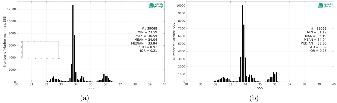
Figure 2: Histograms of SSS from Marine mammals (a) and Aquarius SSS L4 OI v5 - Monthly (IPRC) (b) considering all match-up pairs per bins of 0.1 over the SMOS coastal zone (<800km) 60N-60S Pi-MEP region and for the full satellite product period.
