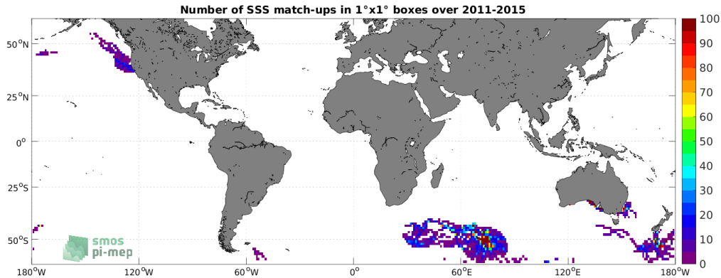
Figure 4: Number of SSS match-ups between Marine mammals SSS and the Aquarius SSS L4 OI v5 - Monthly (IPRC) SSS product for the SMOS coastal zone (<800km) 60N-60S Pi-MEP region over 1^\circ \times 1^\circ boxes and for the full satellite product period.
