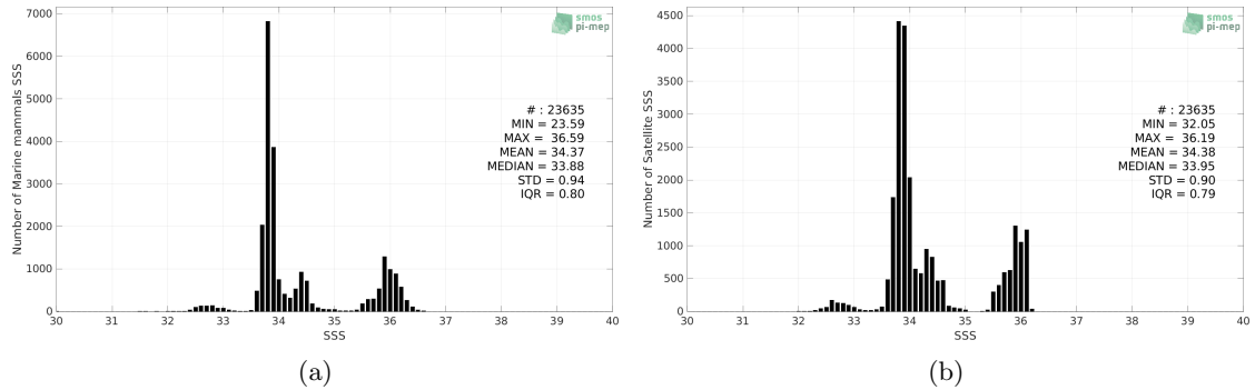
Figure 2: Histograms of SSS from Marine mammals (a) and Aquarius SSS L4 OI v5 - Monthly (IPRC) (b) considering all match-up pairs per bins of 0.1 over the SMOS coastal zone (<800km) 60N-60S Pi-MEP region and for the full satellite product period.
