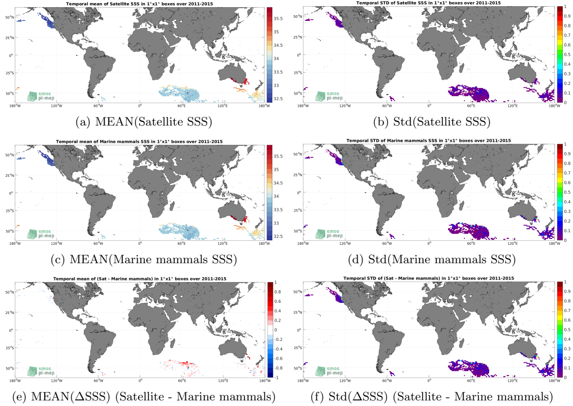
Figure 6: Temporal mean (left) and Std (right) of SSS from Aquarius SSS L4 OI v5 - Monthly (IPRC) (top), Marine mammals (middle), and of \Delta SSS (Satellite - Marine mammals). Only match-up pairs are used to generate these maps.
