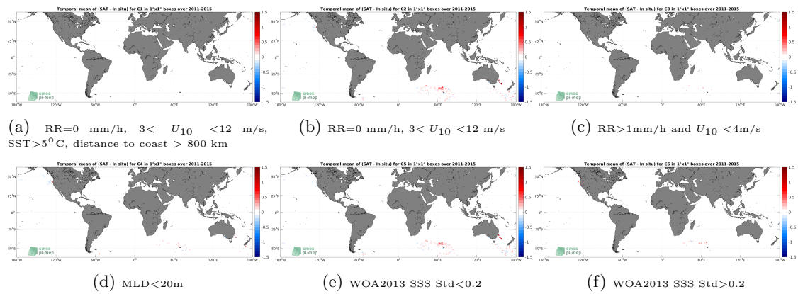
Figure 12: Temporal mean gridded over spatial boxes of size 1^\circ \times 1^\circ of \Delta SSS (Aquarius SSS L4 OI v5 - Monthly (IPRC) - Marine mammals) for 6 different subdatasets corresponding to:RR=0 mm/h, 3 < U_{10} < 12 m/s, SST >5^\circ C, distance to coast > 800 km (a), RR=0 mm/h, 3 < U_{10} < 12 m/s (b), RR >1 mm/h and U_{10} < 4 m/s (c),MLD <20 m (d),WOA2013 SSS Std <0.2 (e),WOA2013 SSS Std >0.2 (f).
