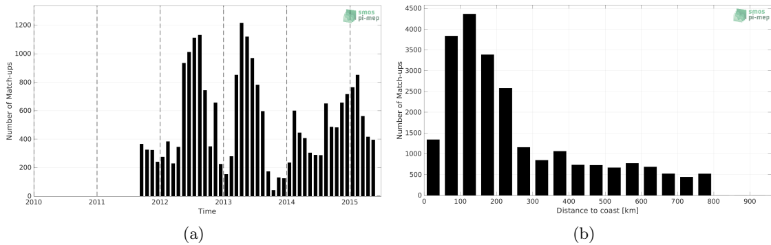
Figure 1: Number of match-ups between Marine mammals and Aquarius SSS L4 OI v5 - Monthly (IPRC) SSS as a function of time (a) and as function of the distance to coast (b) over the SMOS coastal zone (<800km) 60N-60S Pi-MEP region and for the full satellite product period.
