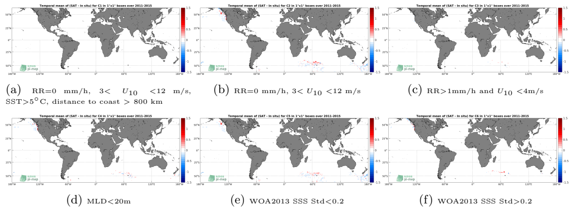
Figure 12: Temporal mean gridded over spatial boxes of size 1^\circ \times 1^\circ of \Delta SSS (Aquarius SSS L4 OI v5 - Monthly (IPRC) - Sea mammals) for 6 different subdatasets corresponding to:RR=0 mm/h, 3 < U_{10} < 12 m/s, SST > 5^\circ\text{C} , distance to coast > 800 km (a), RR=0 mm/h, 3 < U_{10} < 12 m/s (b), RR > 1 mm/h and U_{10} < 4 m/s (c),MLD < 20 m (d),WOA2013 SSS Std < 0.2 (e),WOA2013 SSS Std > 0.2 (f).
