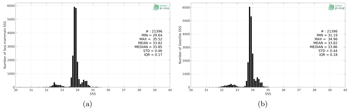
Figure 2: Histograms of SSS from Sea mammals (a) and Aquarius SSS L4 OI v5 - Monthly (IPRC) (b) considering all match-up pairs per bins of 0.1 over the SMOS coastal zone (<800km) 60N-60S Pi-MEP region and for the full satellite product period.
