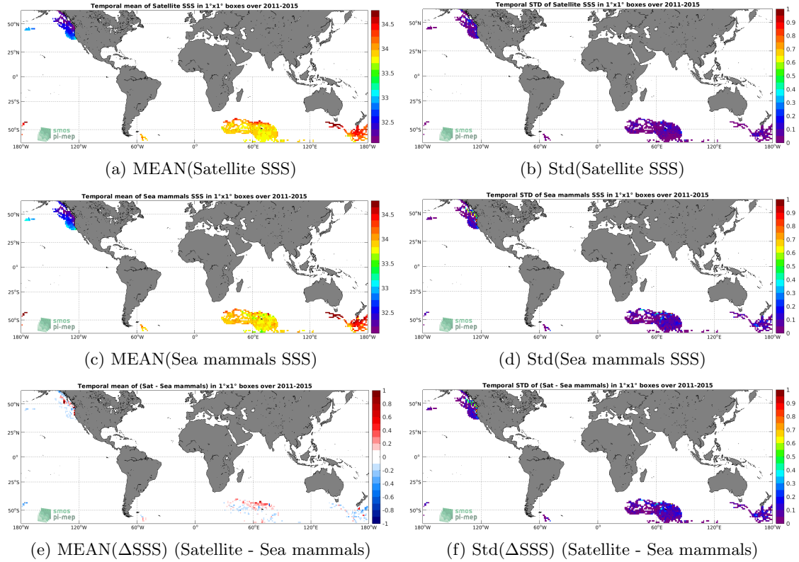
Figure 6: Temporal mean (left) and Std (right) of SSS from Aquarius SSS L4 OI v5 - Monthly (IPRC) (top), Sea mammals (middle), and of \Delta SSS (Satellite - Sea mammals). Only match-up pairs are used to generate these maps.
