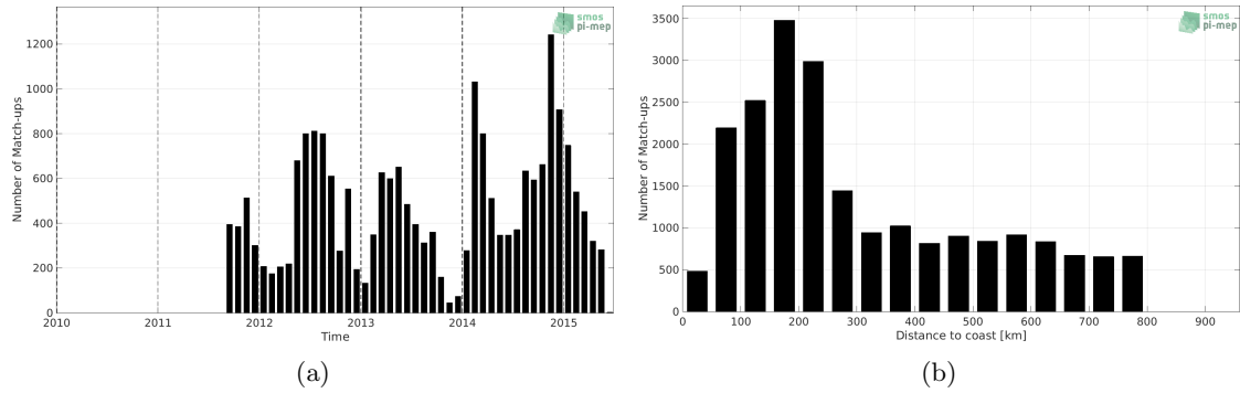
Figure 1: Number of match-ups between Sea mammals and Aquarius SSS L4 OI v5 - Monthly (IPRC) SSS as a function of time (a) and as function of the distance to coast (b) over the SMOS coastal zone (<800km) 60N-60S Pi-MEP region and for the full satellite product period.
