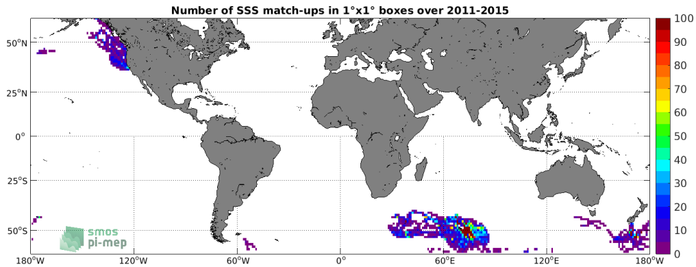
Figure 4: Number of SSS match-ups between Sea mammals SSS and the Aquarius SSS L4 OI v5 - Monthly (IPRC) SSS product for the SMOS coastal zone (<800km) 60N-60S Pi-MEP region over 1°x1° boxes and for the full satellite product period.
