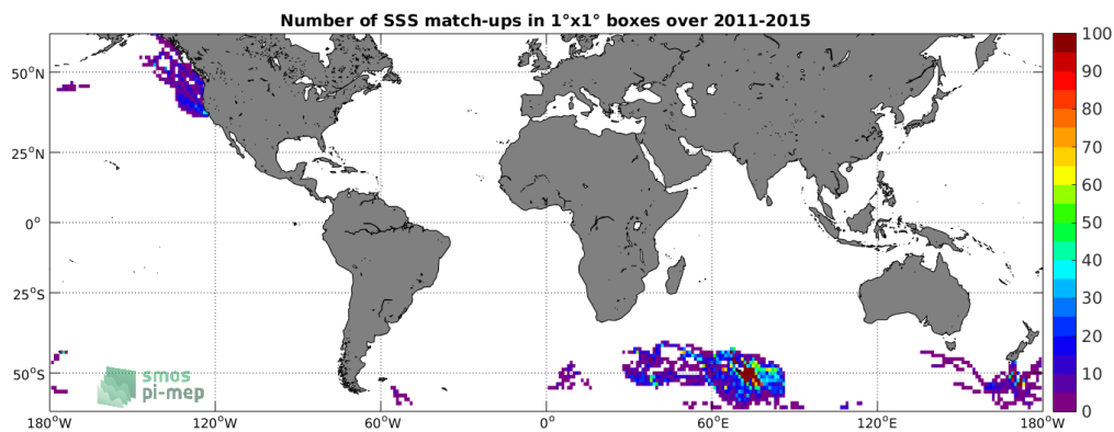
Figure 4: Number of SSS match-ups between Sea mammals SSS and the Aquarius-L4-IPRC-V5-MONTHLY SSS product for the SMOS coastal zone ( \approx 800\text{km} ) 60N-60S Pi-MEP region over 1^\circ \times 1^\circ boxes and for the full satellite product period.
