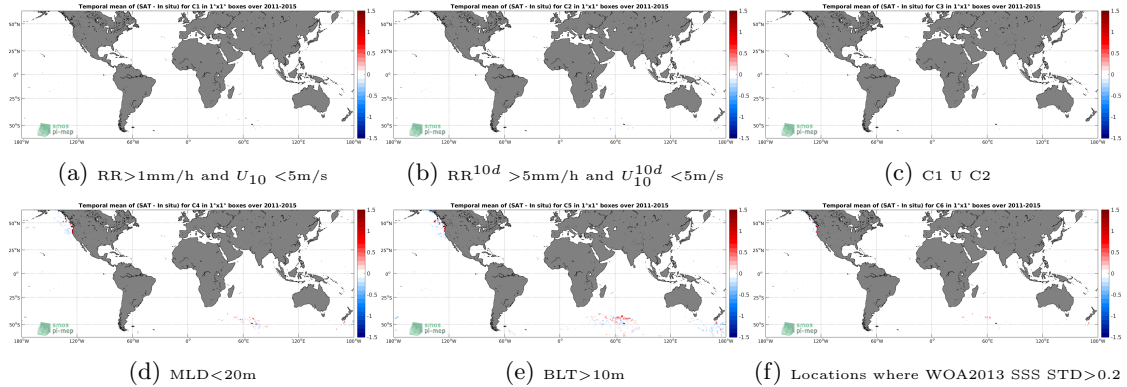
Figure 12: Temporal mean gridded over spatial boxes of size 1°x1° of \Delta SSS (Aquarius-L4-IPRC-V5-MONTHLY - Sea mammals) for 6 different subdatasets corresponding to:RR>1mm/h and U_{10} < 5 m/s (a), RR^{10d} > 5 mm/h and U_{10}^{10d} < 5 m/s (b), C1 U C2 (c),MLD<20m (d),BLT>10m (e),Locations where WOA2013 SSS STD>0.2 (f).
