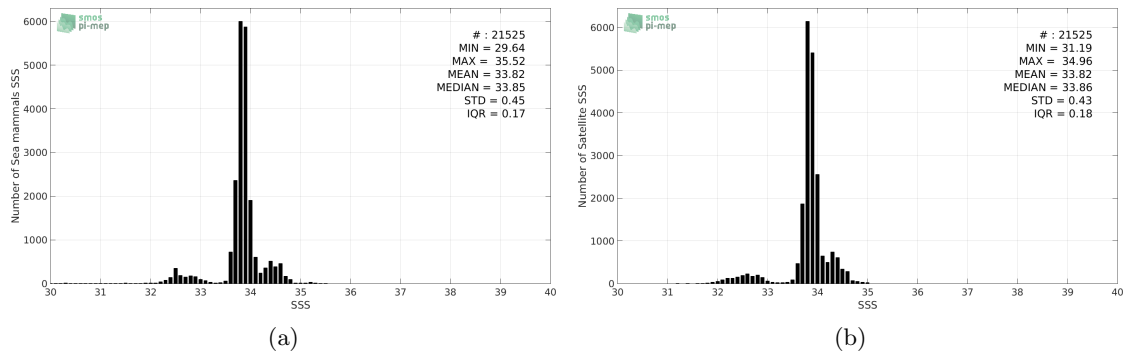
Figure 2: Histograms of SSS from Sea mammals (a) and Aquarius-L4-IPRC-V5-MONTHLY (b) considering all match-up pairs per bins of 0.1 over the SMOS coastal zone ( \geq 800\text{km} ) 60N-60S Pi-MEP region and for the full satellite product period.
