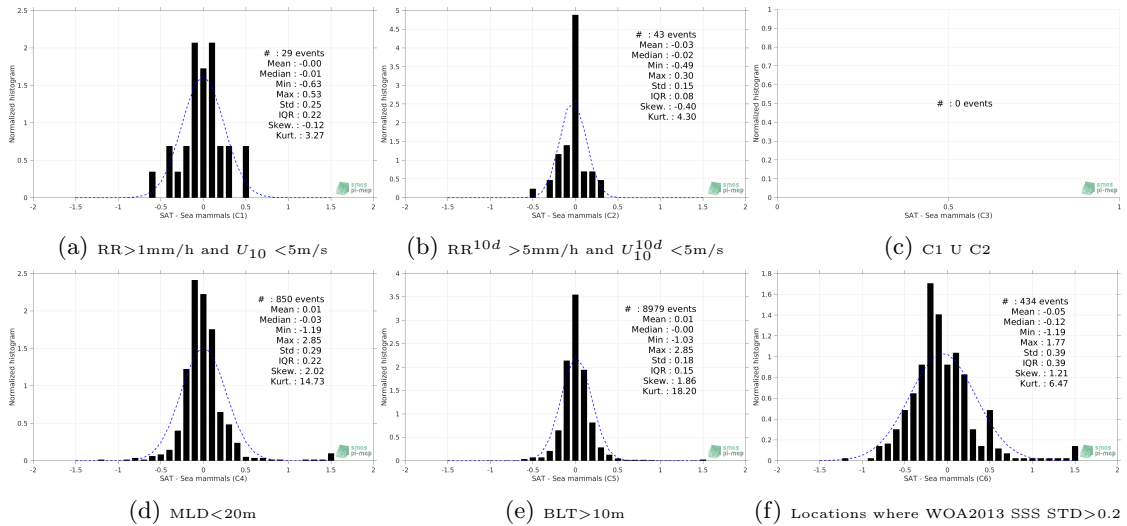
Figure 13: Normalized histogram of \Delta SSS (Aquarius-L4-IPRC-V5-MONTHLY - Sea mammals) for 6 different subdatasets corresponding to: RR>1mm/h and U_{10} < 5 m/s (a), RR^{10d} > 5 mm/h and U_{10}^{10d} < 5 m/s (b), C1 U C2 (c),MLD<20m (d),BLT>10m (e),Locations where WOA2013 SSS STD>0.2 (f).
